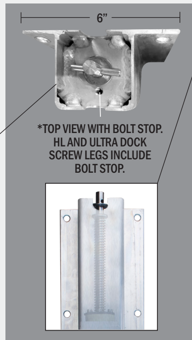
3" x 3" Tube with 6" Wide Flange
