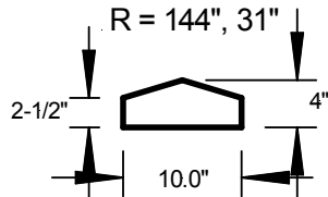
WC - 45 L = 36 R = 144", 31"
