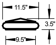
WC - 46T L = 24", TL = 32"
