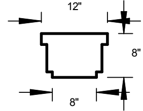
WC - 04T L = 24"
