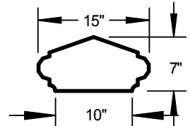
DWC 10T L = 32"
