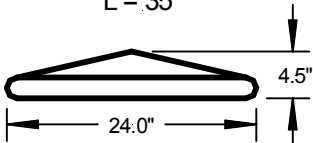
WCB - 24T L = 35"
