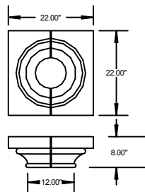
CC - 62008 Cap for 12" column
