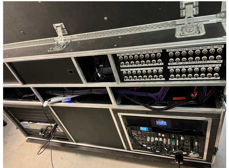
Rear View of FLYPACK1 showing Presonus StudioLive Mixer, Ubiquity Network Switches, and I/O panel.
