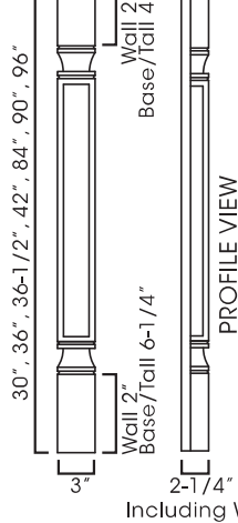
POLE75-XXXX HALF LEG
