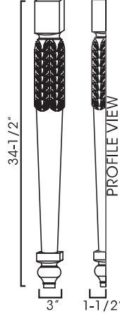
LEG83* HALF LEG
