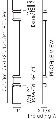
LEG28 B3X3 (SL ONLY ) FULL LEG
