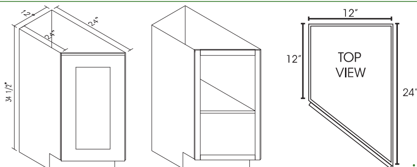
BASE TRANSITIONAL LEFT SHOWN
