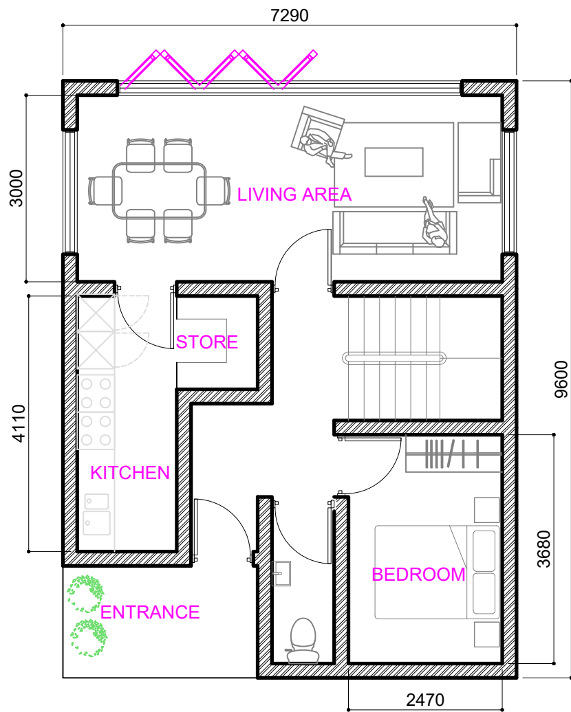
GROUND FLOOR
