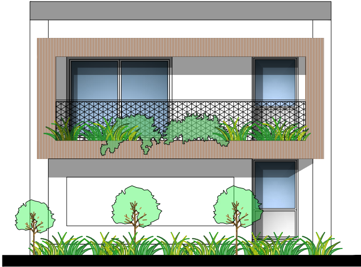
PROPOSED RIGHT ELEVATION. 1:100
