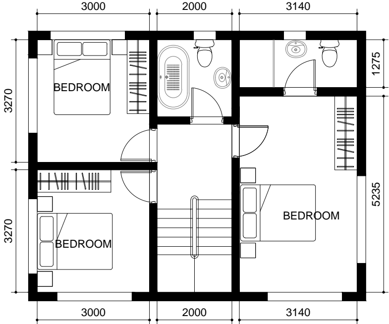
PROPOSED FIRST FLOOR PLAN. 1:100
