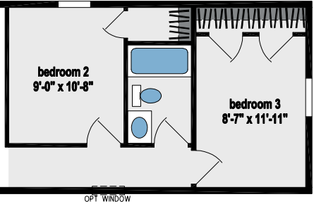
OPTION 2 BEDROOM CONFIGURATION
