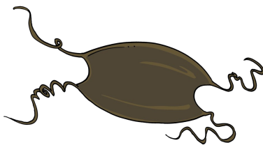
dogfish egg case
