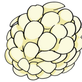
whelk egg case
