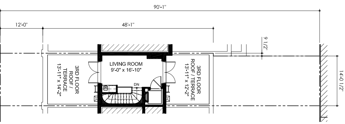
PENTHOUSE
