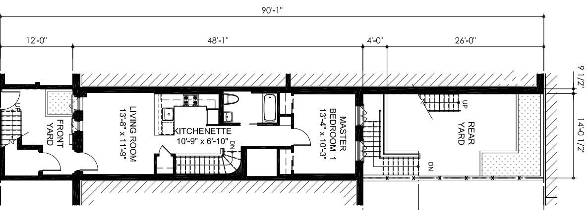
GROUND FLOOR
