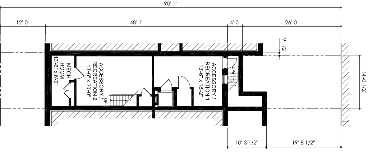
RECREATION FLOOR
