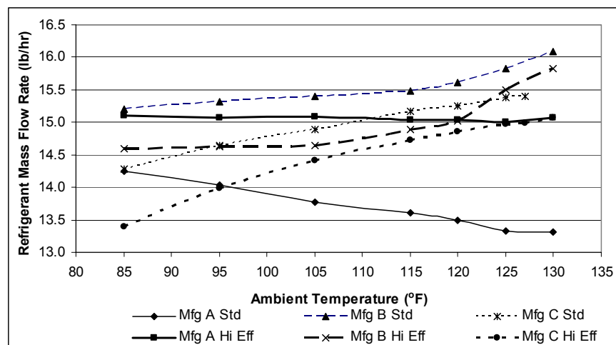
Figure 7. Refrigerant Mass Flow Rate Based on RTTC Test Data for All Six Standard and High Efficiency Units Subject to Various Ambient Temperatures
