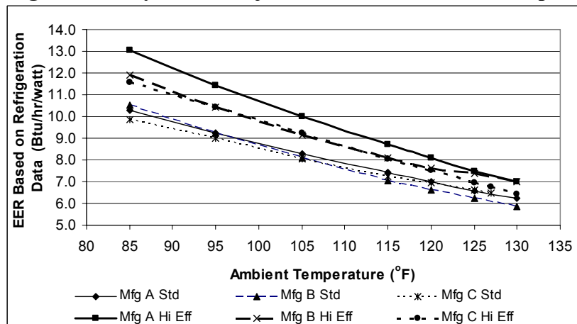
Figure 8. EERs Based on RTTC Refrigeration Side Test Data for All Six Standard and High Efficiency Units Subject to Various Ambient Temperatures
