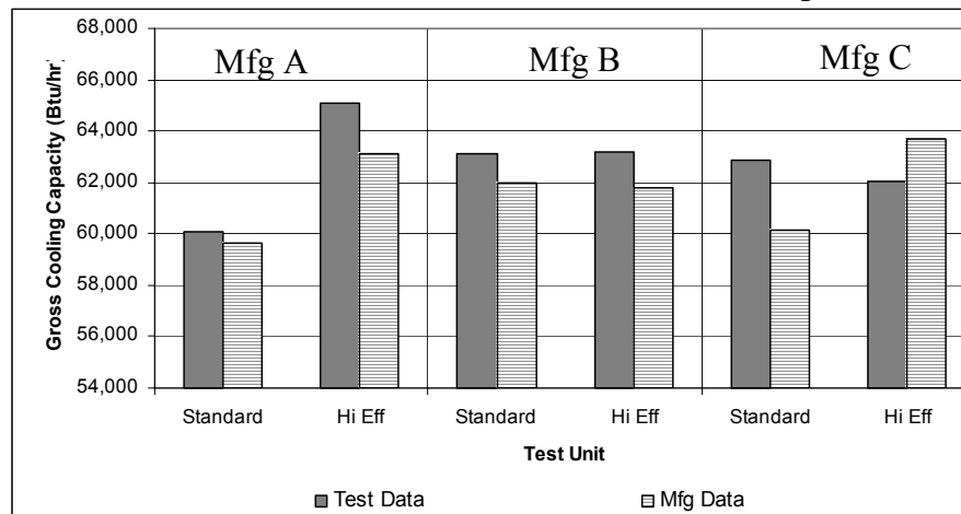
Figure 2. Comparison of Gross Cooling Capacity from Manufacturers Published Data and RTTC Test Data Based on 95°F Ambient Temperature
