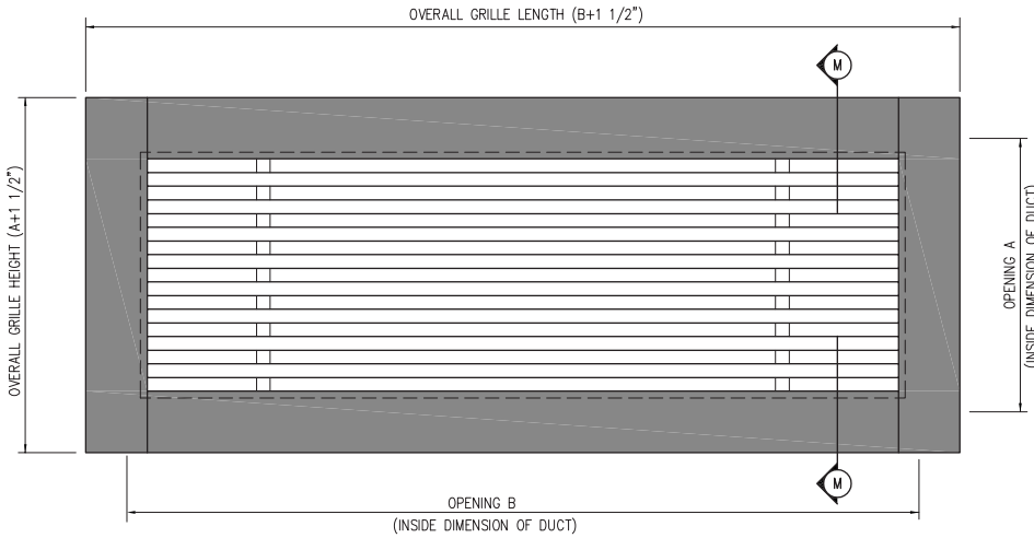
PLAN VIEW SCALE: 6'-0"=1'-0"
