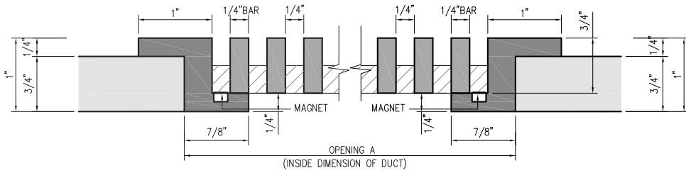
(M) SECTION DETAIL SCALE: 1"=1'-0"
