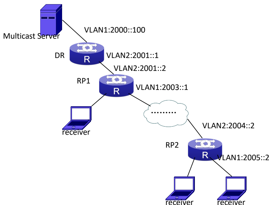
Figure 12-13 The ANYCAST RP v6 function of a router
