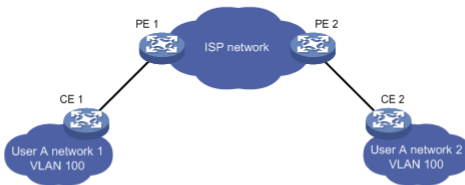
Figure 2-12 BPDU Tunnel application
