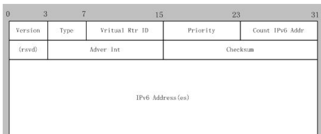
Figure 12-20 VRRPv3 message
