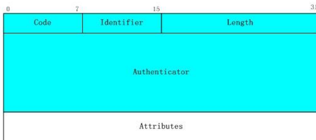
Figure 6-211 Message structure for RADIUS
