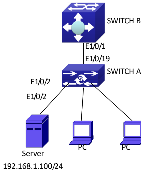
Figure 3-6 ARP scanning prevention typical configuration example
