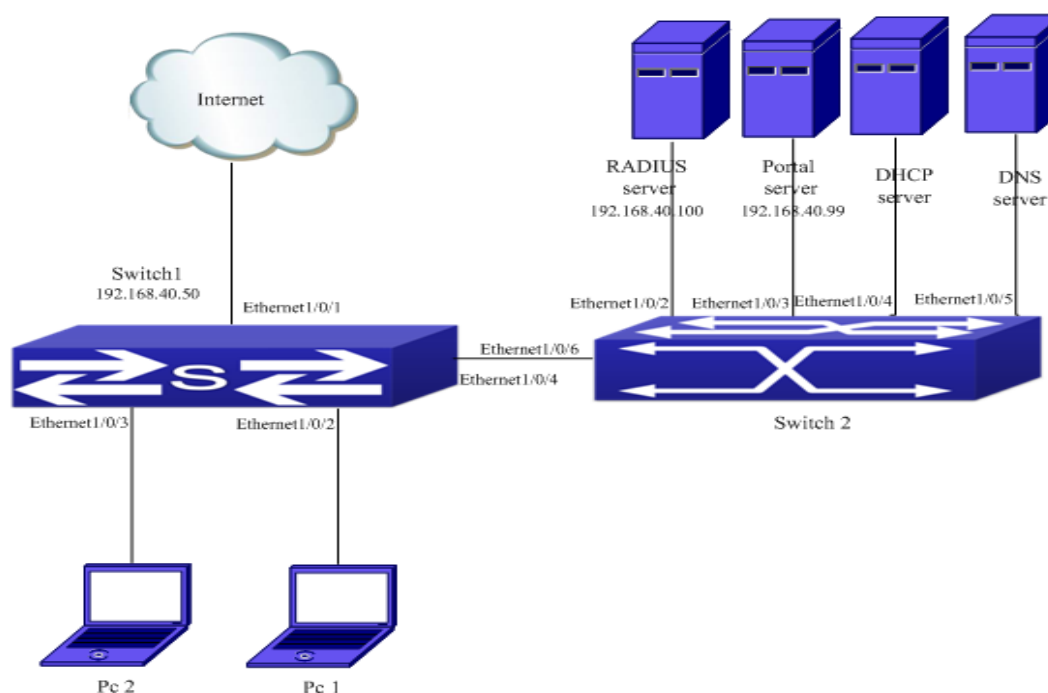
Figure 6-28 accounting function configuration
