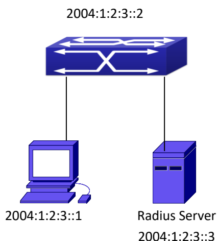
Figure 6-17 IPv6 Radius
