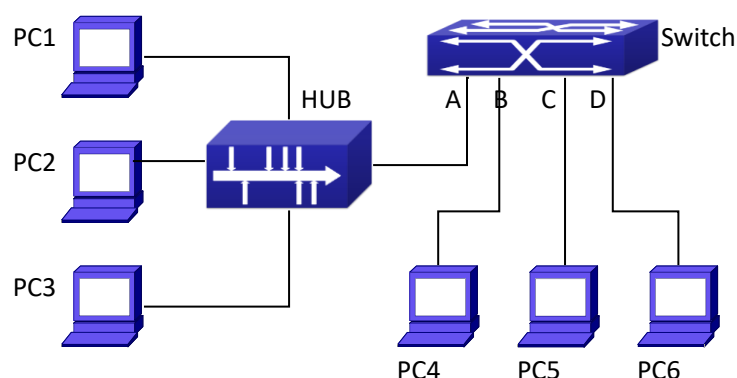
Figure 3-8 ARP GUARD schematic diagram
