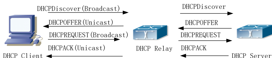
Figure 3-15 DHCP relay
