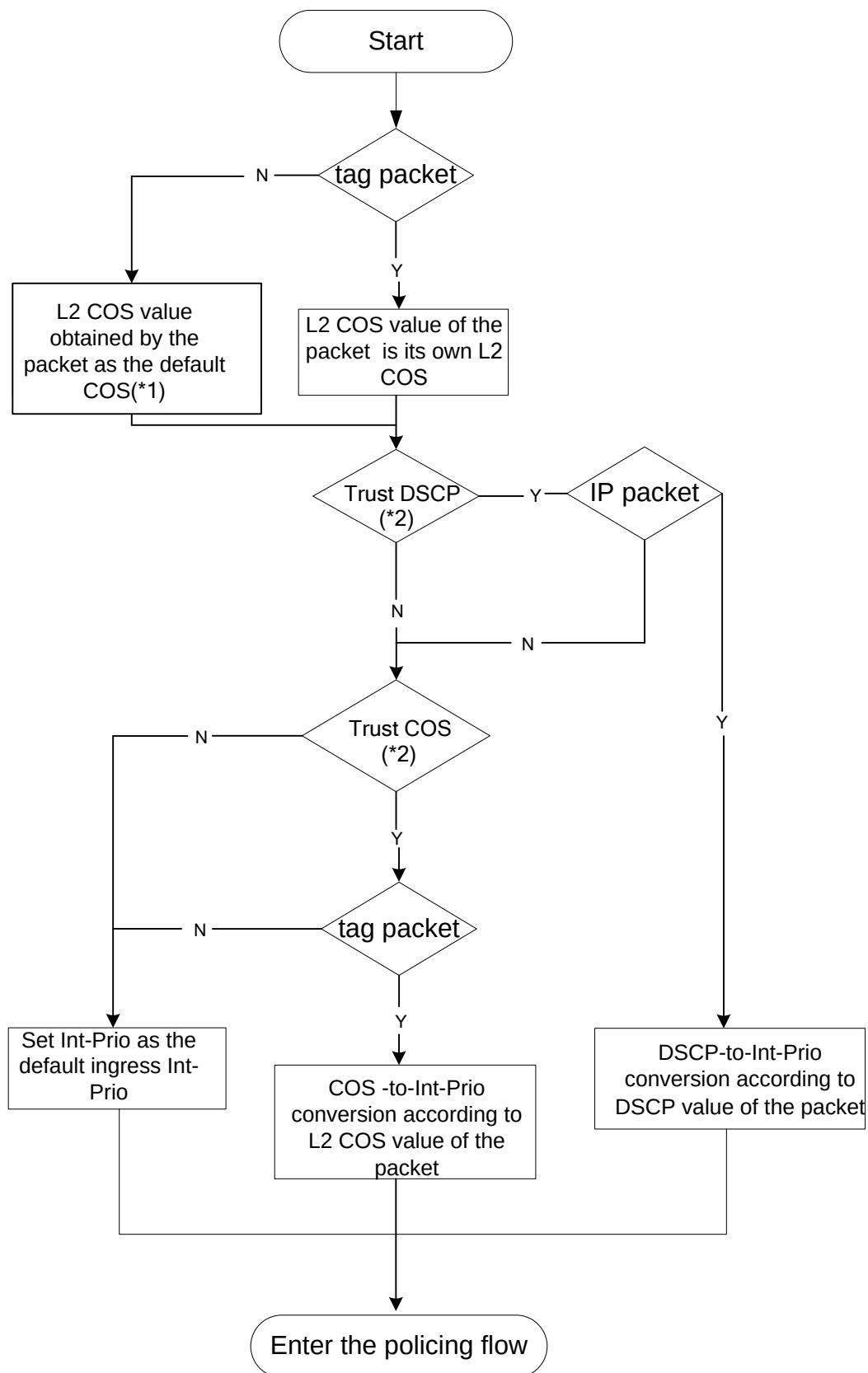
Figure 6-37 Classification process
