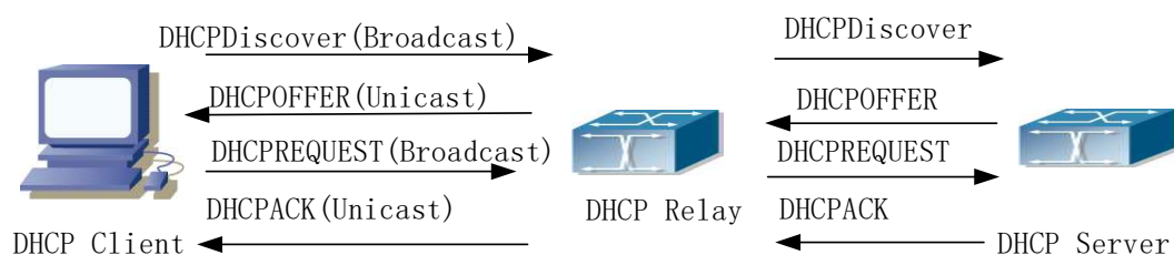
Figure 3-10 DHCP relay
