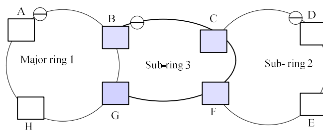
Figure 7-19 the interconnection ring topology without virtual channel
