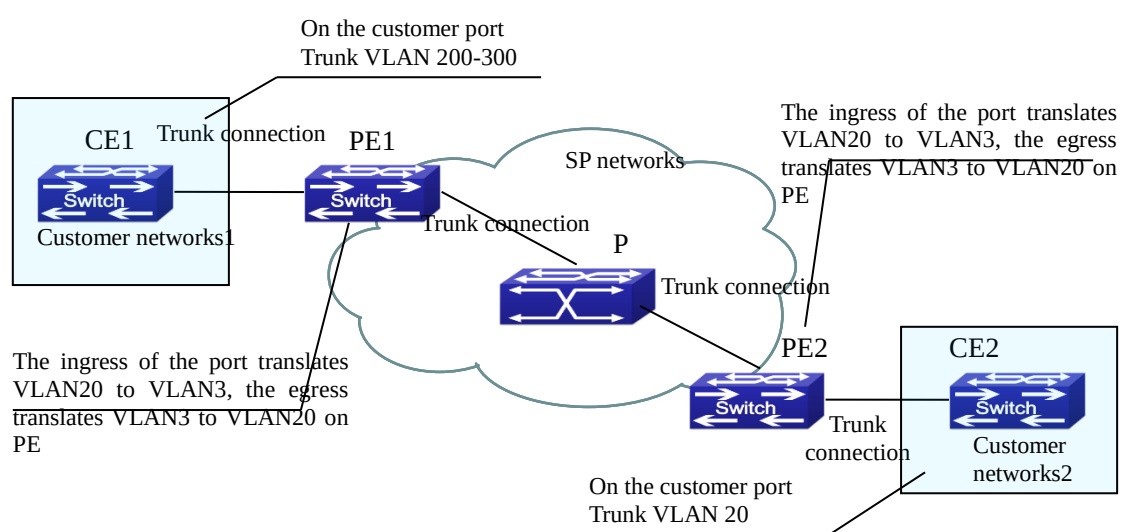
Figure 2-32 Vlan translation topology mode
