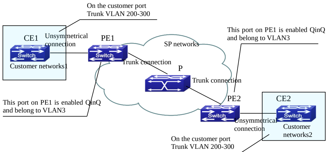
Figure 2-30 Dot1q-tunnel based Internetworking mode
