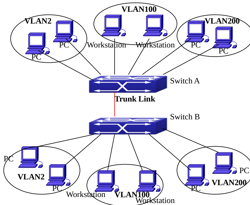
Figure 2-26 Typical VLAN Application Topology
