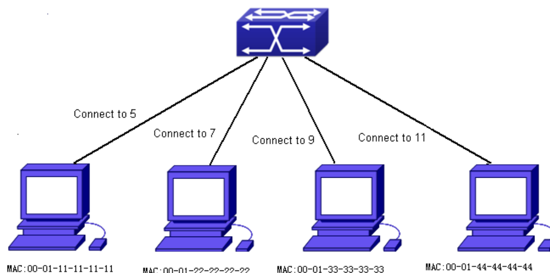
Figure 2-38 MAC Table typical configuration example
