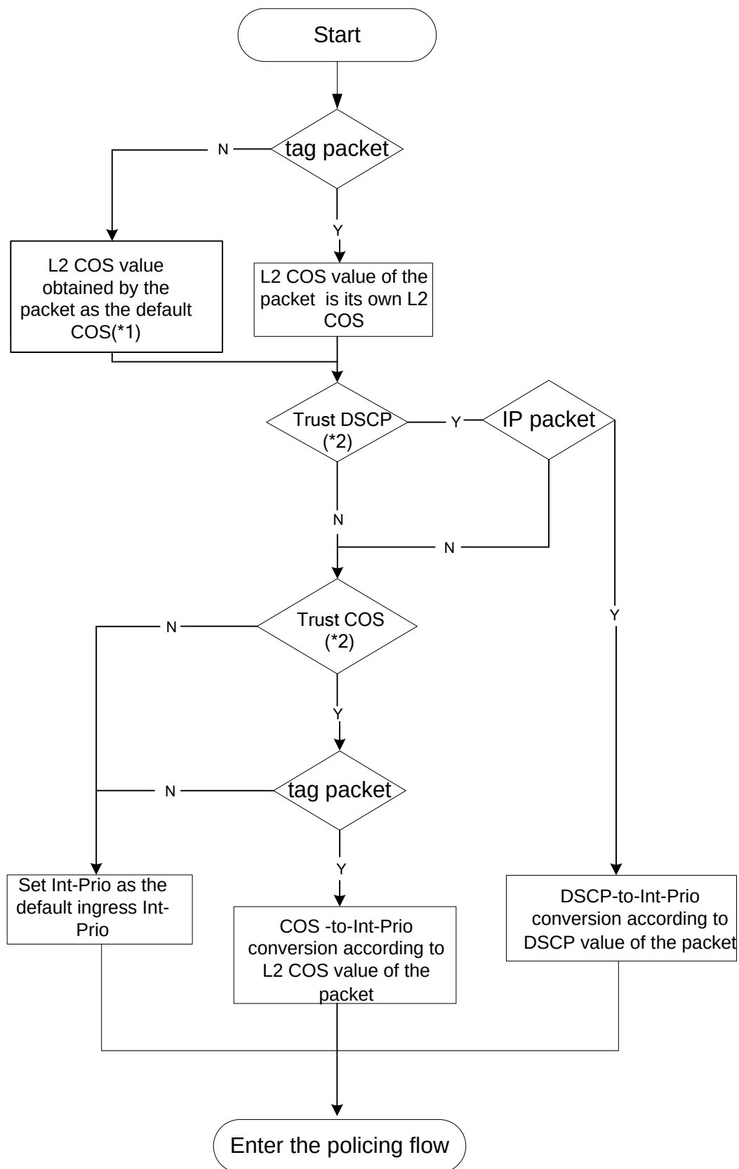
Figure 5-47 Classification process
