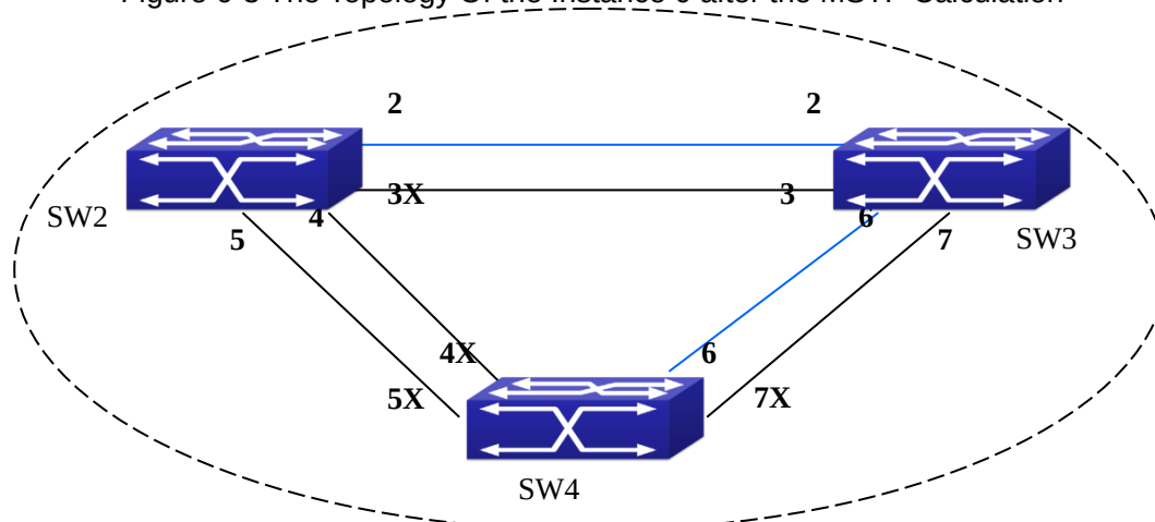
Figure 6-3 The Topology Of the Instance 0 after the MSTP Calculation
