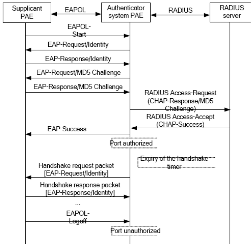
Figure 5-12 the Authentication Flow of 802.1x EAP Termination Mode
