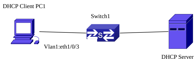
Figure 3-15 DHCP option 82 typical application example
