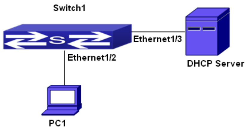
Figure 3-10 DHCP configuration example
