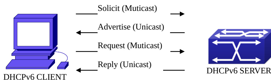
Figure 10-1 DHCPv6 negotiation
