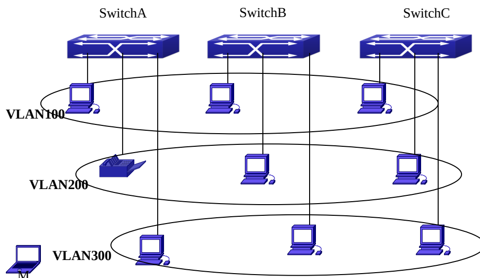
Figure 2-33 Typical topology application of dynamic VLAN
