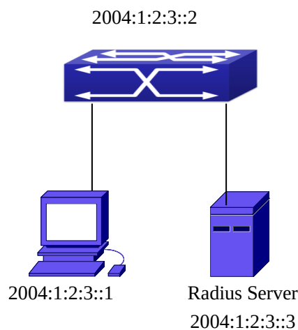
Figure 5-20 IPv6 Radius
