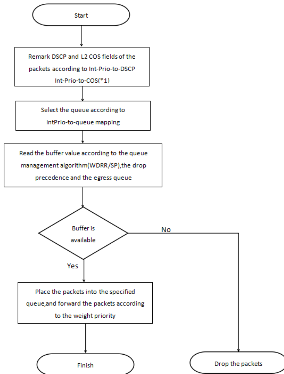
Figure 5-49 Queuing and Scheduling process
