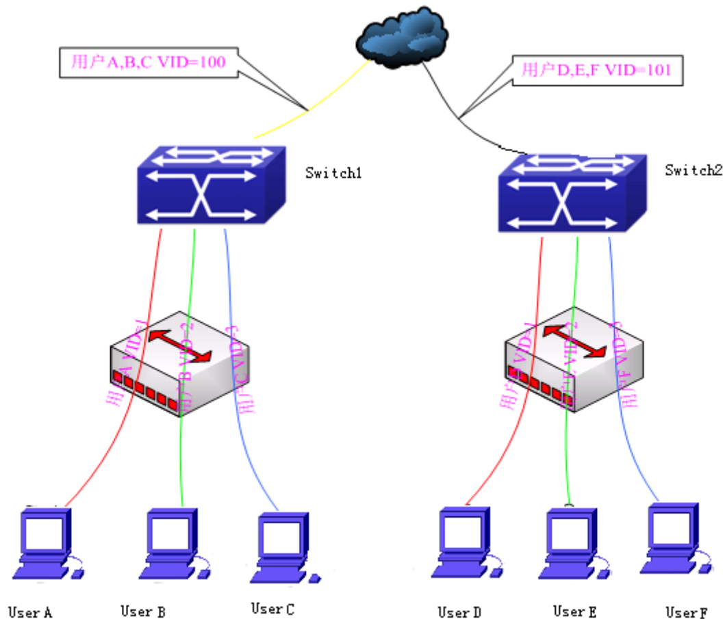
Figure 2-36 VLAN-translation typical application
