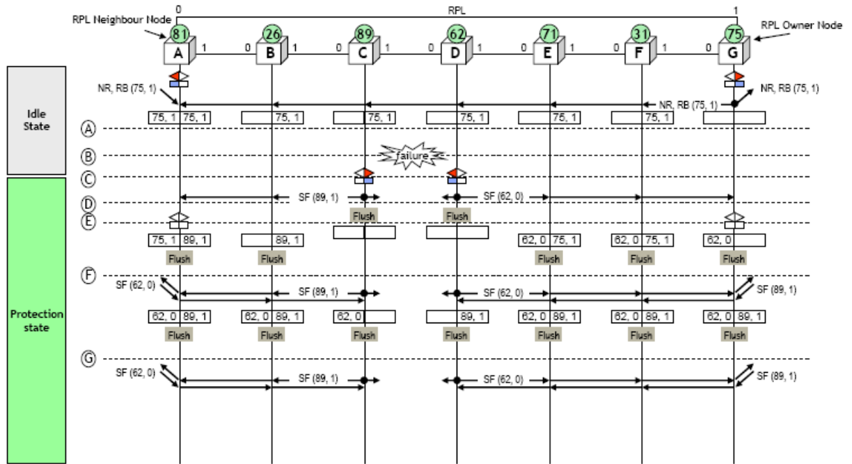
Figure 6-6 single-link fault
