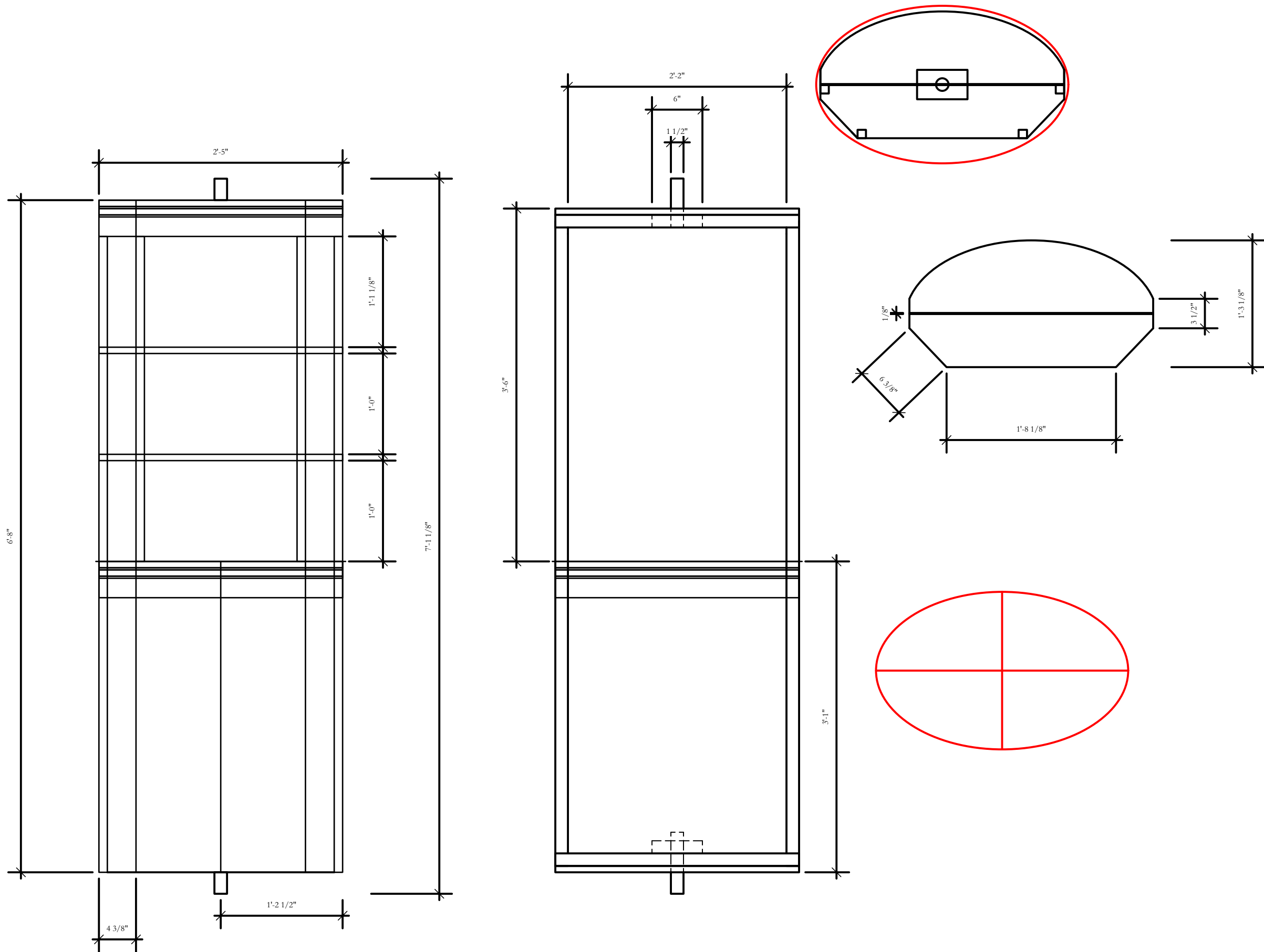
Little Shop of Horrors - Rotating Cabinet Drafted and constructed by Nicky Tomlin 1" = 1' - 00"
