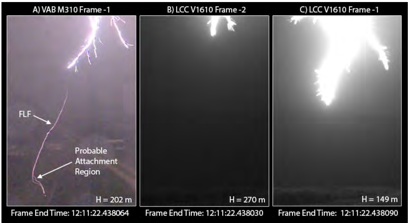
Fig. 4. Event 4 high-speed video images recorded on August 30, 2015 at 12:11:22.438, A) VAB M310 pre-return stroke frame showing FLF, B-C) consecutive LCC V1610 pre-return stroke frames not showing FLF.
