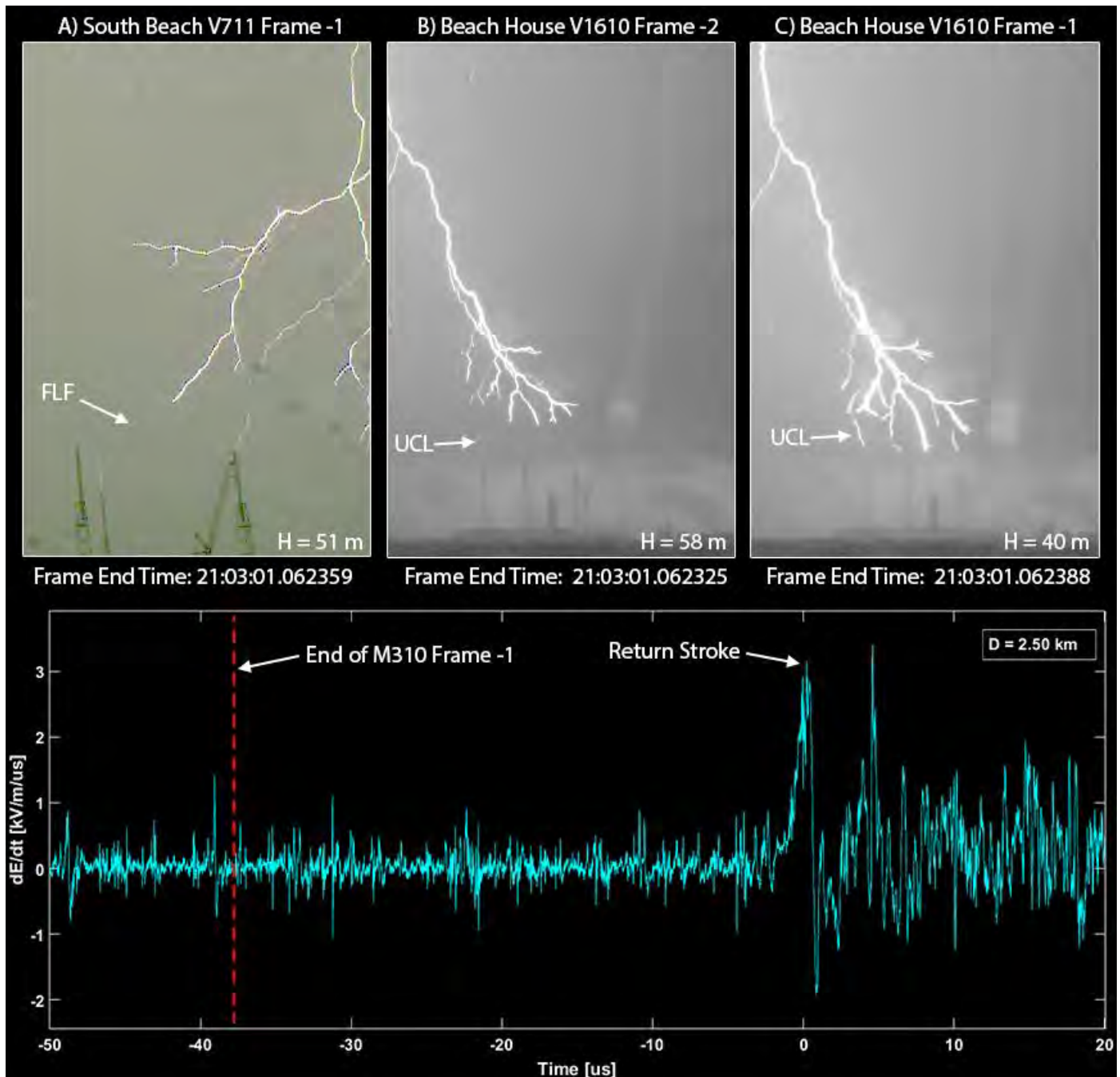
Fig. 5. Event 5 high-speed video images and dE/dt waveforms recorded on October 11, 2015 at 21:03:01.062 A) South Beach V711 pre-return stroke frame showing FLF and multiple unconnected upward leaders, B-C) consecutive Beach House V1610 pre-return stroke frames not showing FLF, but showing both a UCL and multiple unconnected upward leaders.
