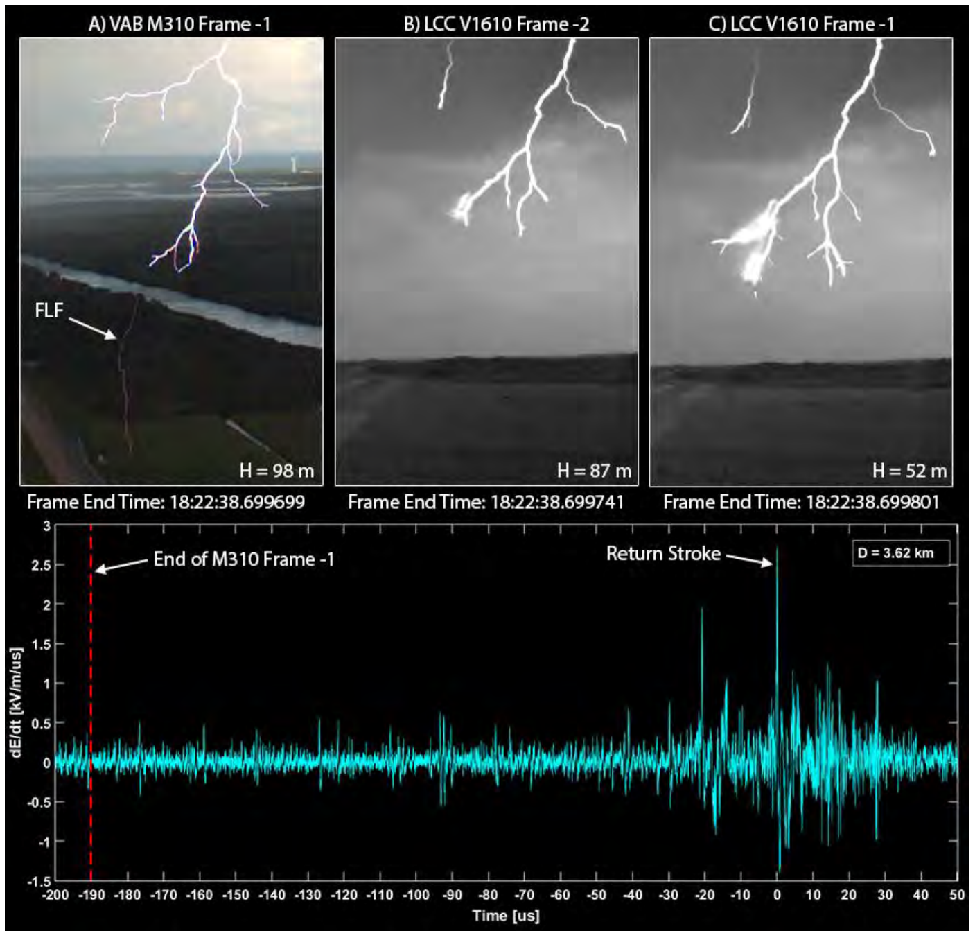
Fig. 1. Event 1 high-speed video images and dE/dt waveforms recorded on August 20, 2015 at 18:22:38.699 (UT), A) VAB M310 pre-return stroke frame showing FLF, B-C) consecutive LCC V1610 pre-return stroke frames not showing FLF.
