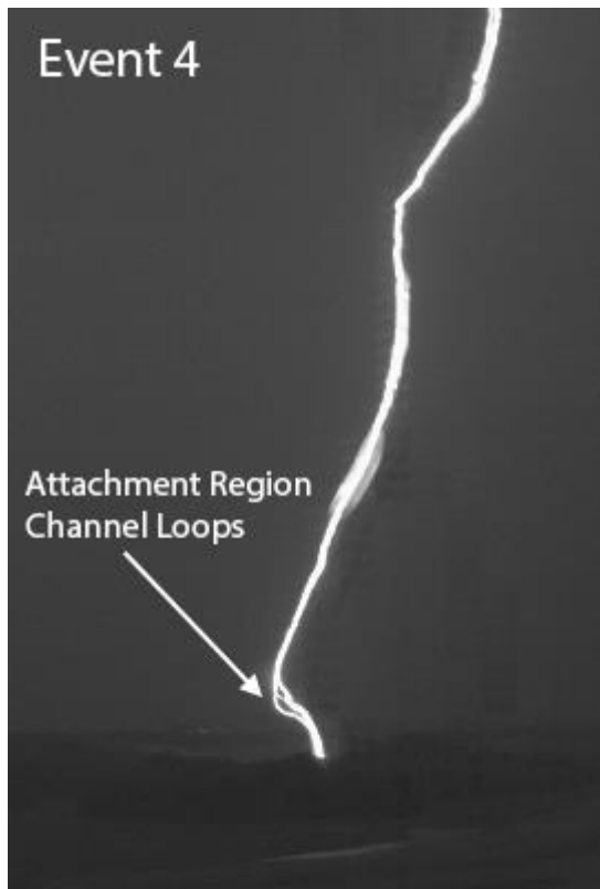
Fig. 6. Post return-stroke LCC V1610 frame recorded during Event 4 on August 30, 2015 at 12:11:22.438 showing channel loops from 17-33 m above ground level. The channel loops are typically indicative of the region where the attachment process occurred.
