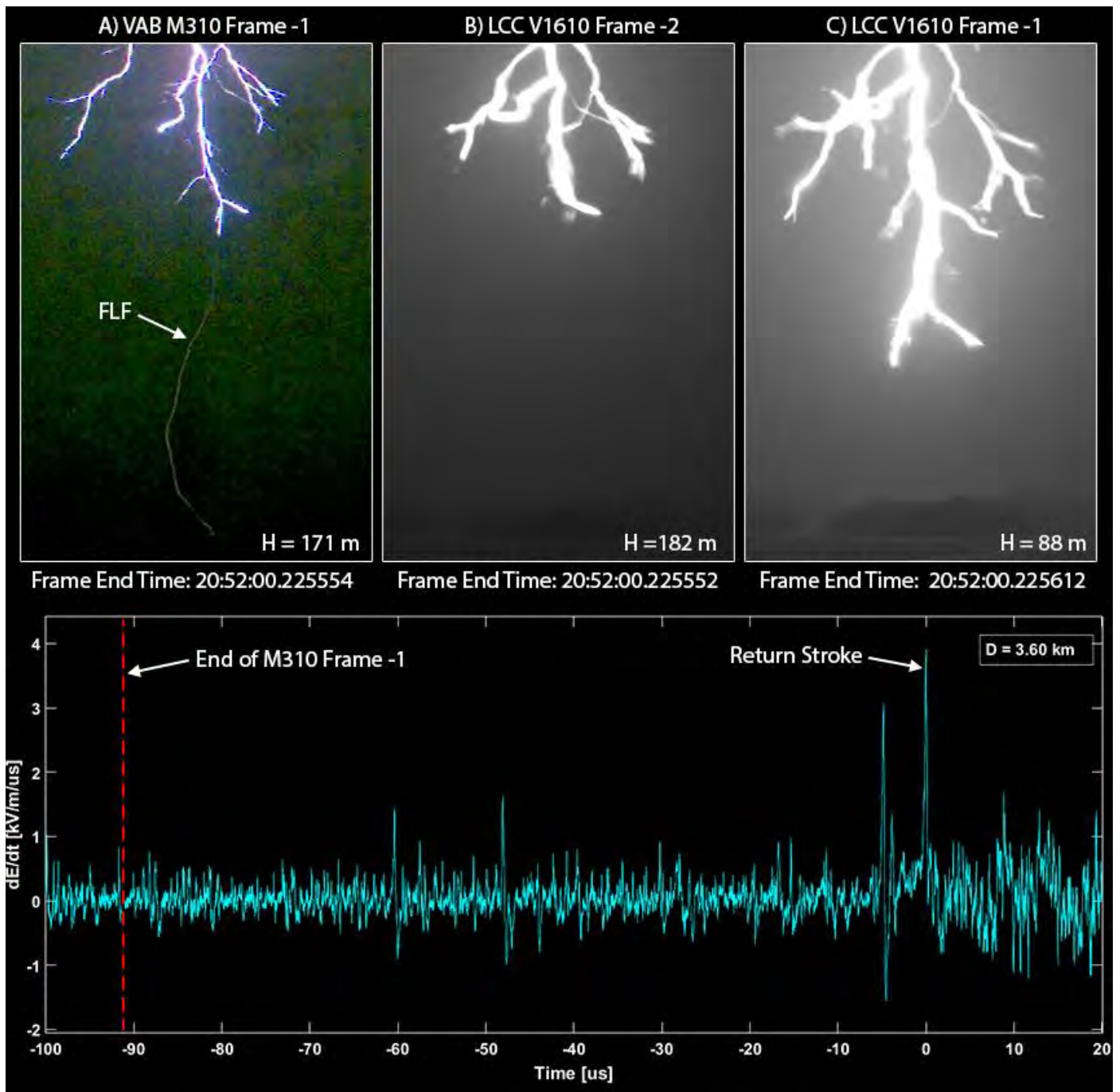
Fig. 3. Event 3 high-speed video images and dE/dt waveforms recorded on August 26, 2015 at 20:52:00.225, A) VAB M310 pre-return stroke frame showing FLF, B-C) consecutive LCC V1610 pre-return stroke frames not showing FLF.
