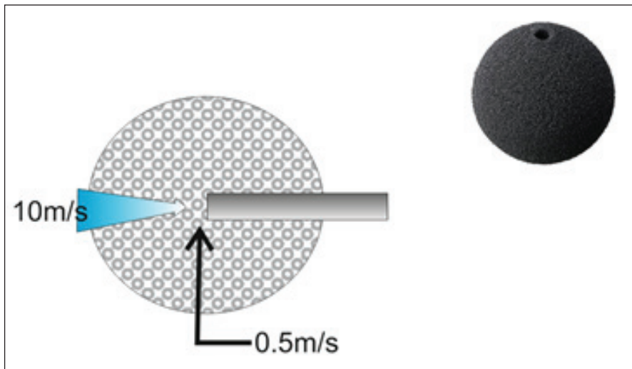
Fig. 8. Windscreen structure.
