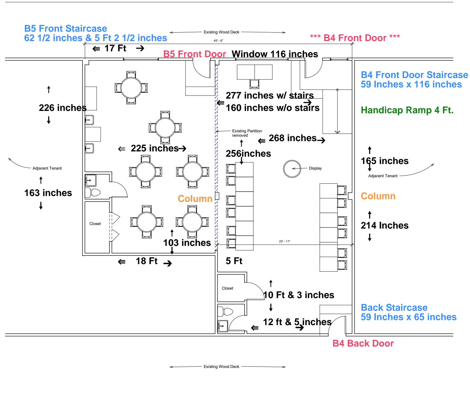
Existing Units B-4 & B-5 Combined Floor Plan
