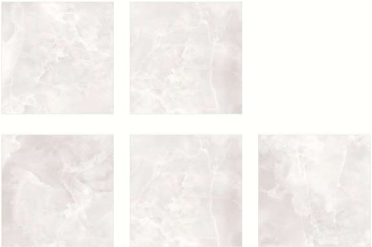
6 RANDOM TILES
