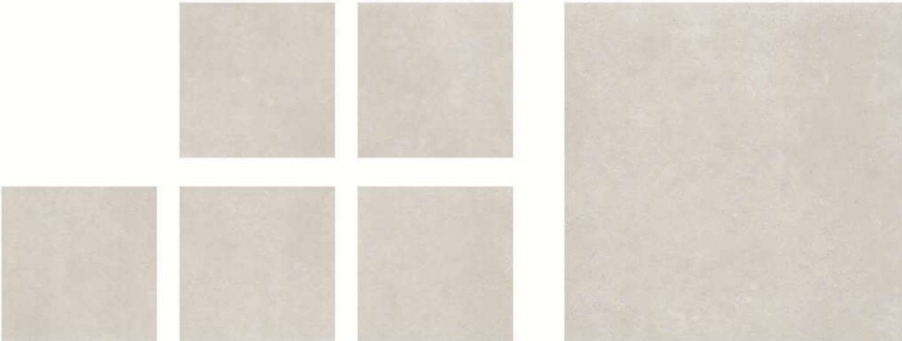
6 RANDOM TILES
