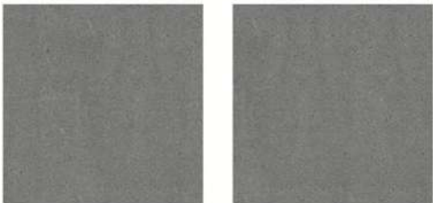
3 RANDOM TILES
