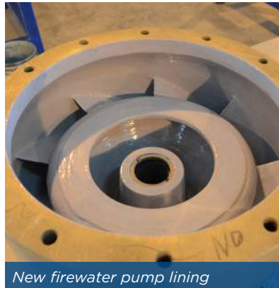
Impeller protected with Belzona lining
