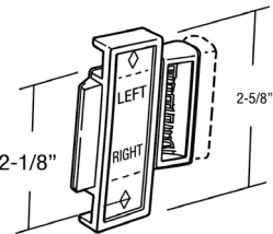
09037 2 Piece Sliding Window Centre Lock with Spring
