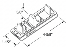
02404 Adjustable Accordion Floor Guide for Sliding Doors
