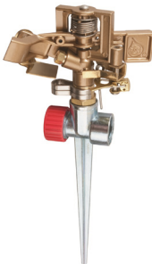
RW-99535C RainWave Pulsating Sprinkler on Metal Spike Base, 85' (26 m) Diameter
