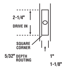
DEADBOLT LATCH
