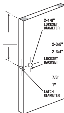
LOCKSET LOCATION
