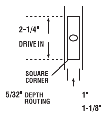
LOCKSET LATCH
