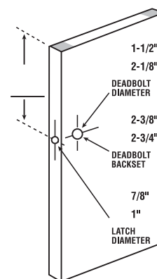
DEADBOLT LOCATION
