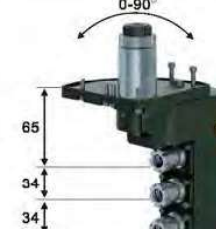
3-spindle drilling/milling unit ⚙
