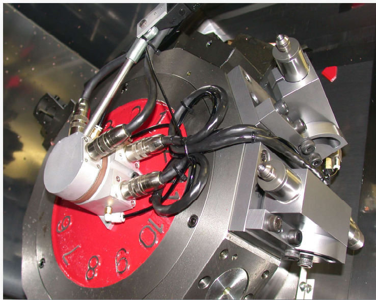
Pictured: NSK E3000 Spindle on a Miyano ABX using a Futureswiss variable angle spindle holder
