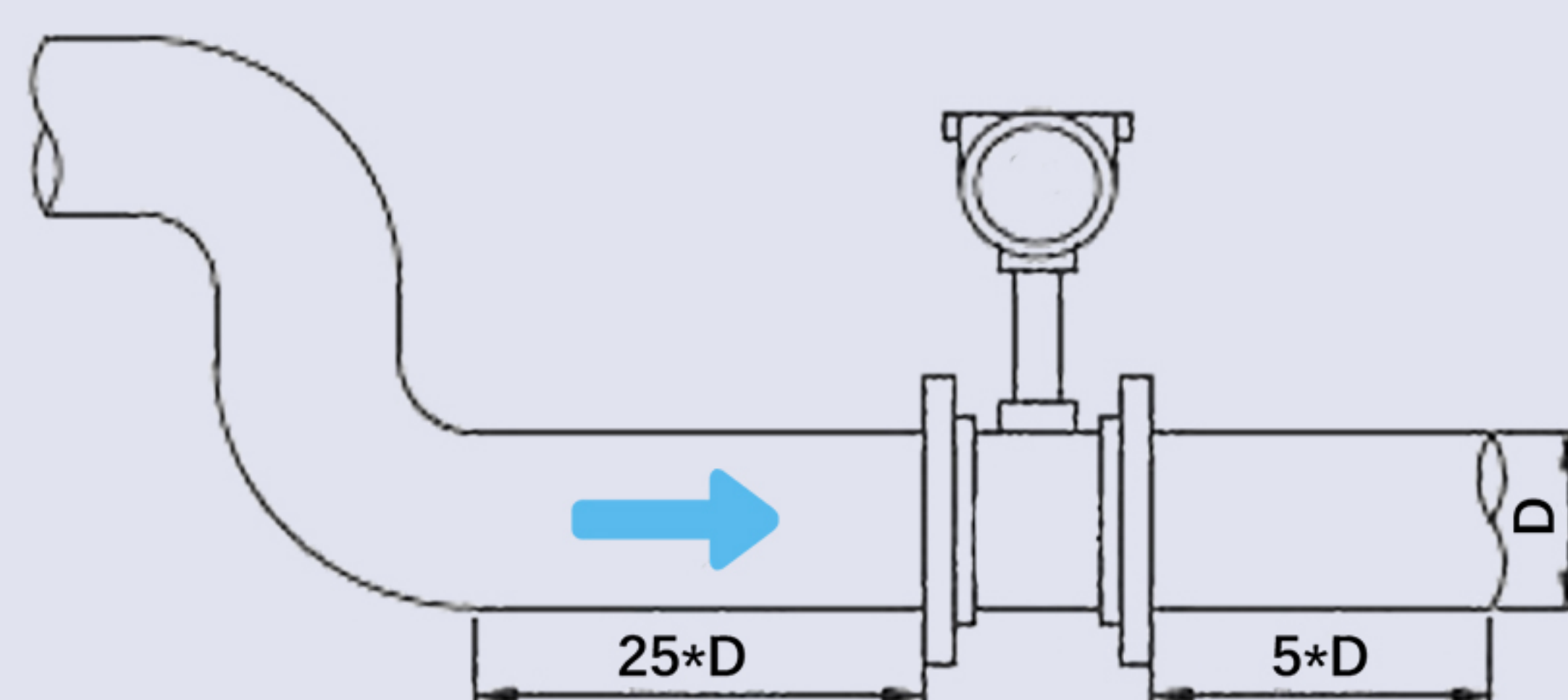
4. 2*90 elbow pipe in same plane
