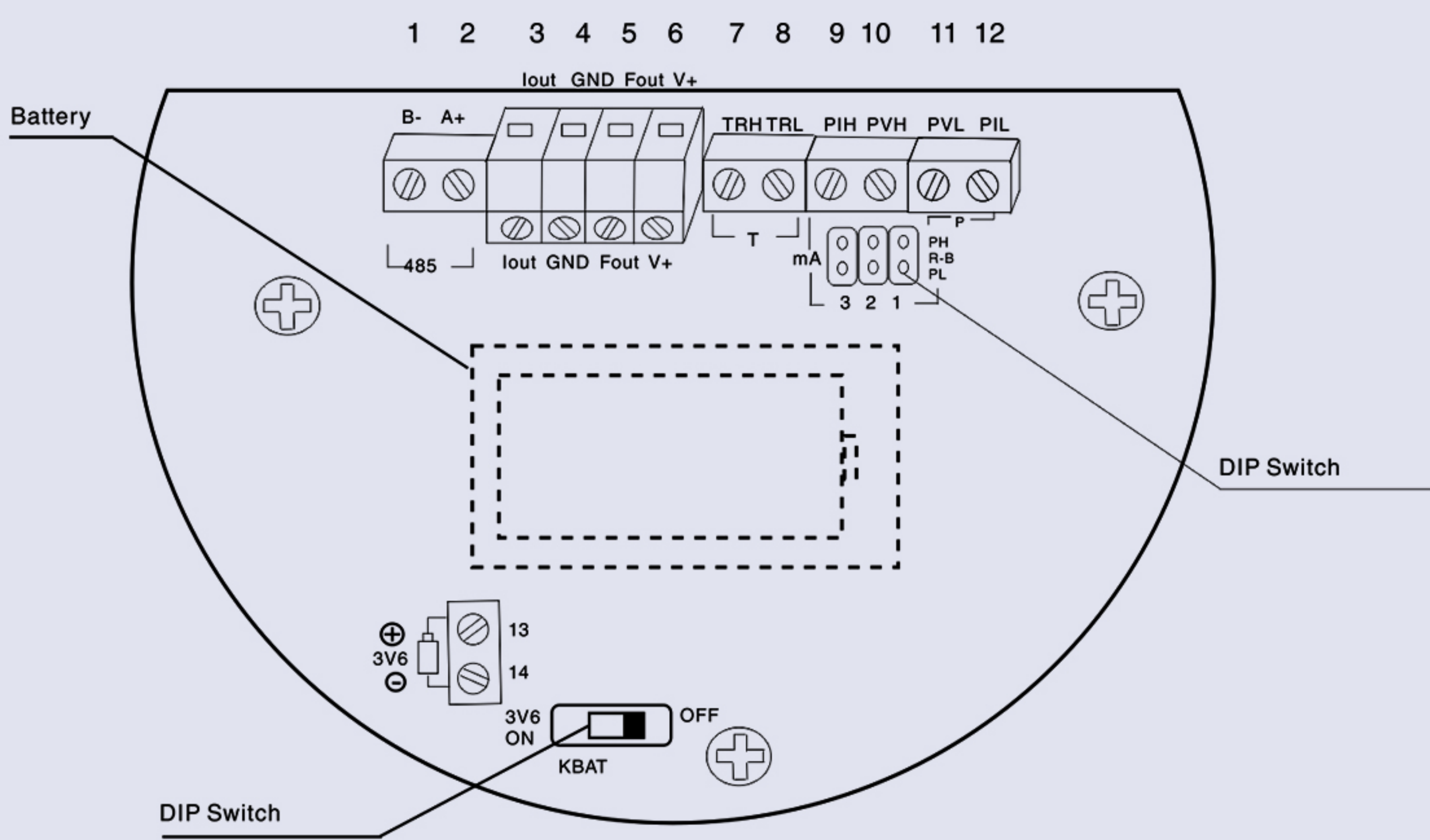
3 wire 4-20mA output terminal board
