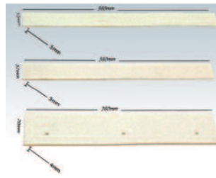
Cleaning felt for PM46 (10/pack) Part# FELTPM46
