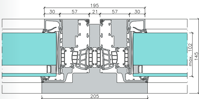
› Horizontal section B - B (Mullion)
