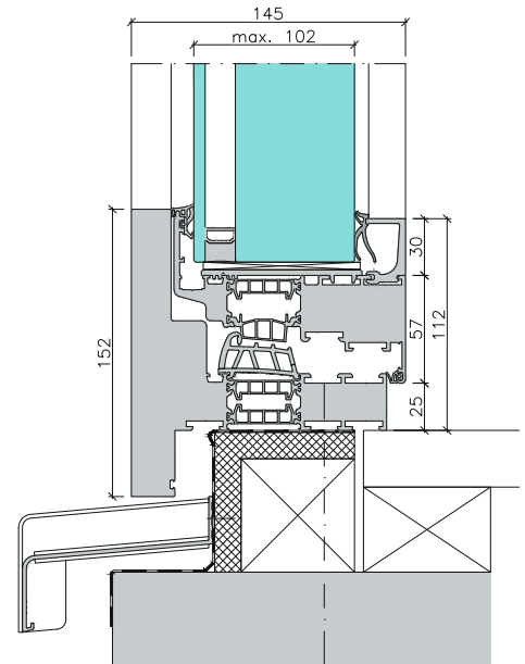
› Vertikal section C - C (Parapet)
