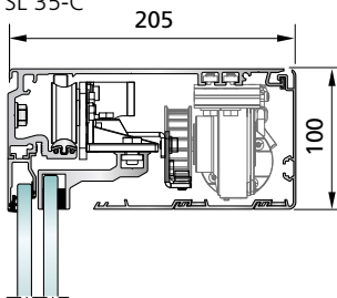
Compact - low-profile frame (PSA) SL 35-C
