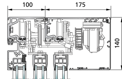
Standard - telescopic thermally insulated (PST) SL 35-T
