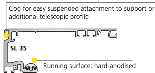
Compact - all glass (PSF) SL 35-C
