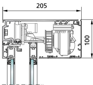
Compact - standard (PSXP) SL 35-C
