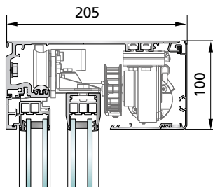
Compact - thermally insulated (PST) SL 35-C
