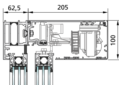
Compact - thermally insulated (PST) SL 35-C
