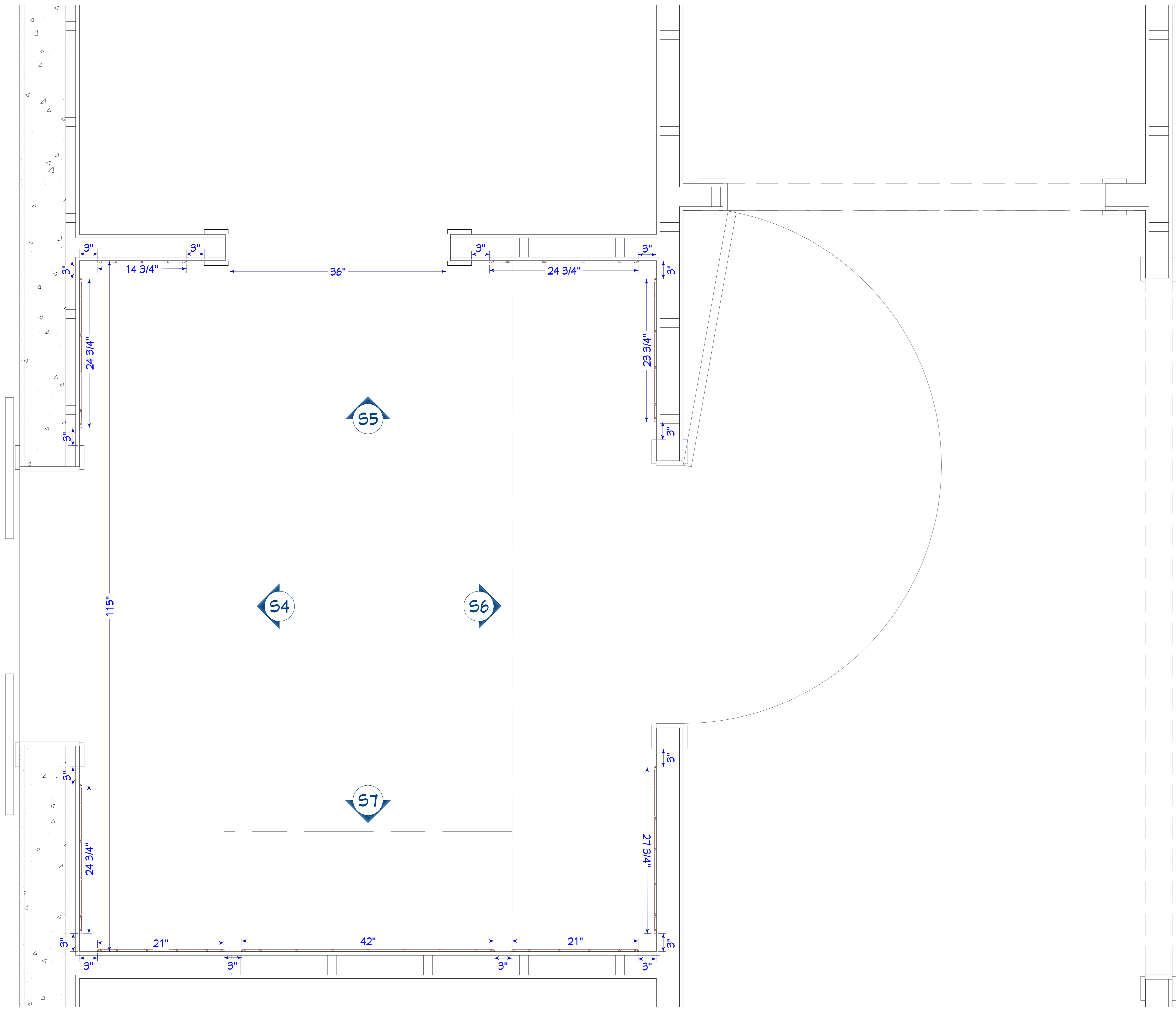
ELEVATOR LOBBY PLAN VIEW
