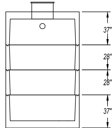
Outlet View
