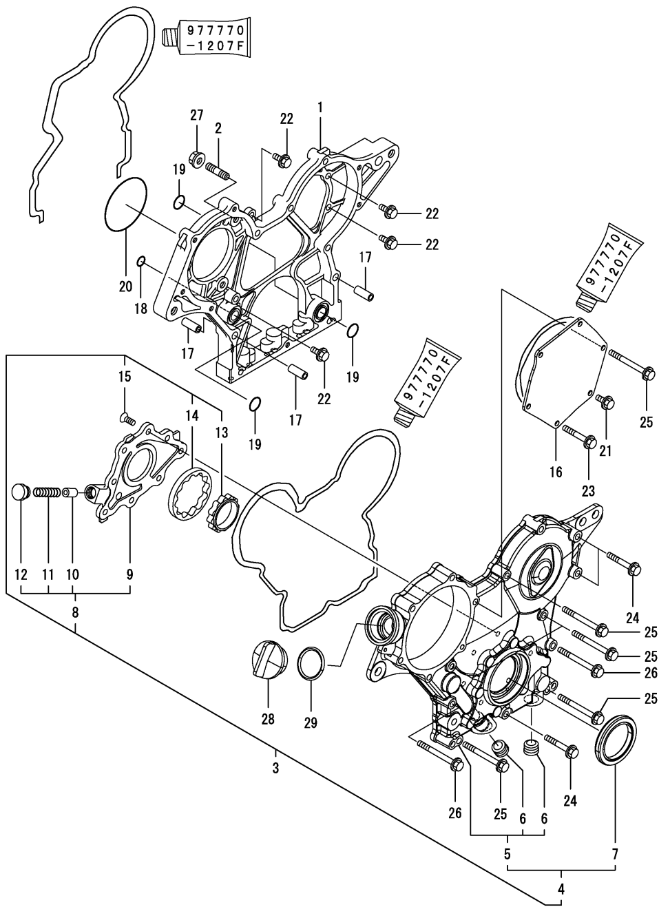
Fig.2. GEAR HOUSING
