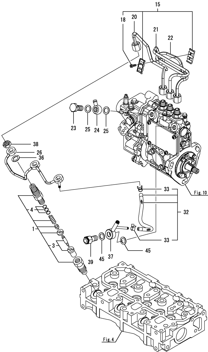
Fig.12. FUEL INJECTION VALVE
