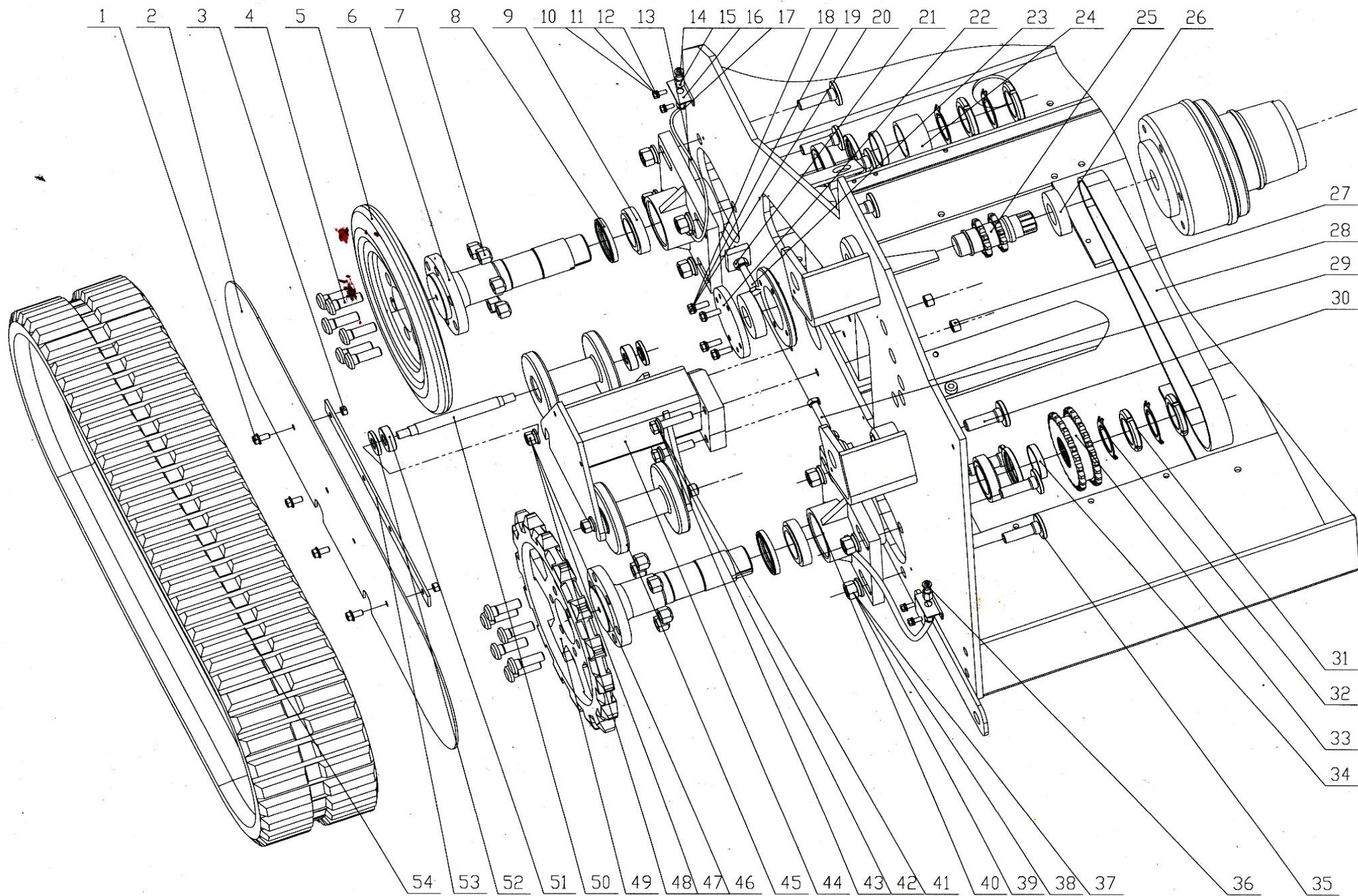
传动总成明细表 (Drive assembly for HY380T)
