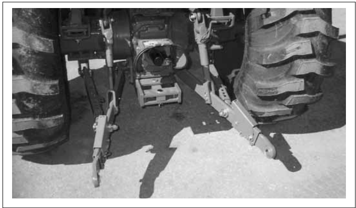
Fig. 25 TRACTOR LOWER LINKS
