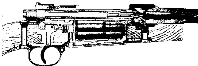
MODEL 98. GERMAN INFANTRY RIFLE. RIGHT SIDE PHANTOM VIEW WITH ARM READY TO FIRE
