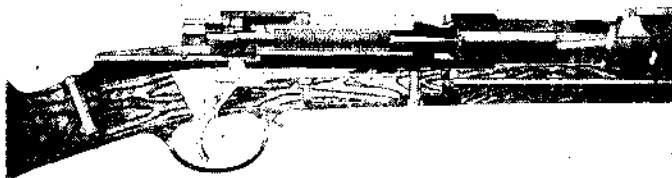
MODEL 78-80 SERBIAN RIGHT SIDE PHANTOM VIEW WITH ACTION CLOSED AND CARTRIDGE IN CHAMBER FIRED
