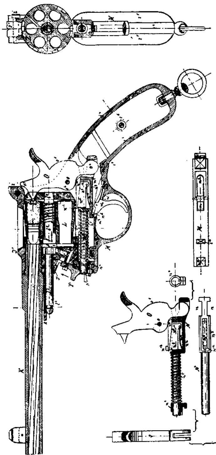
MODEL 78. MAUSER IMPROVED REVOLVER.
