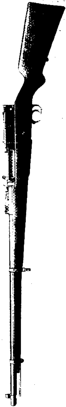
MODEL 96-08, MAUSER SEMI-AUTOMATIC RIFLE. LEFT SIDE VIEW WITH ACTION CLOSED READY TO FIRE.
