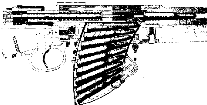
BELGIAN MAUSER WITH 10-SHOT MAGAZINE. PHANTOM RIGHT SIDE VIEW WITH MAGAZINE LOADED AND CARTRIDGE IN CHAMBER READY TO FIRE
