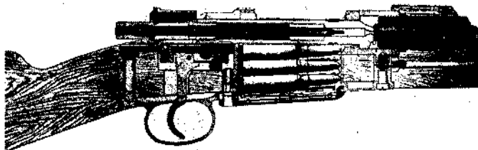
MODEL 93. SPANISH INFANTRY RIFLE. RIGHT SIDE PHANTOM VIEW SHOWING ACTION CLOSED, MAGAZINE AND CHAMBER LOADED
