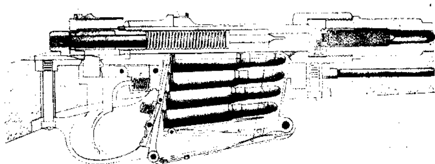
MODEL 90. SPANISH RIGHT SIDE VIEW WITH CHAMBER AND MAGAZINE LOADED
