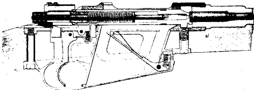
Spanish Model 92-93 Magazine Carbine, Cal. 7 mm. Arm cocked ready to fire cartridge in chamber, magazine empty.
