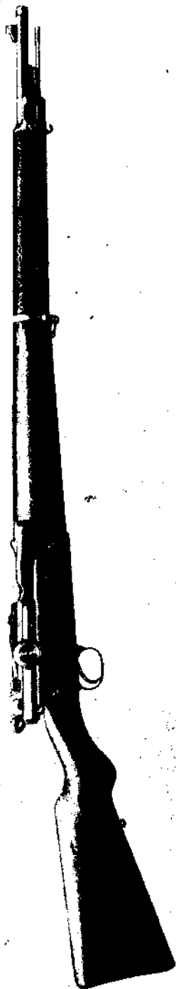
MODEL 98. MAUSER SEMI-AUTOMATIC RIFLE WITH CLAW BLOCK LOCK. SHORT RECOIL SYSTEM.
