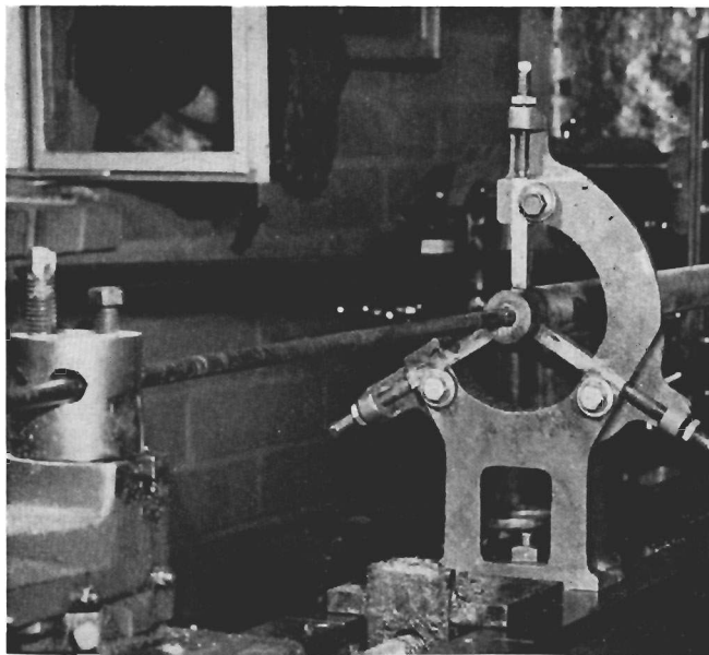
Starting with round solid bar, Hicks drills, reams and rifles barrels entirely within own shop with power tools.
