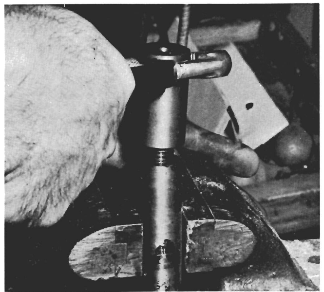
Breech screw plug is fitted before barrel tang which holds barrel in stock is cut and filed from plug end.
