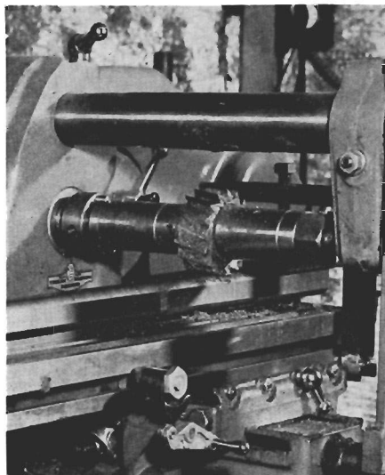
Modern milling machine is used to cut the eight sides of the barrel.
