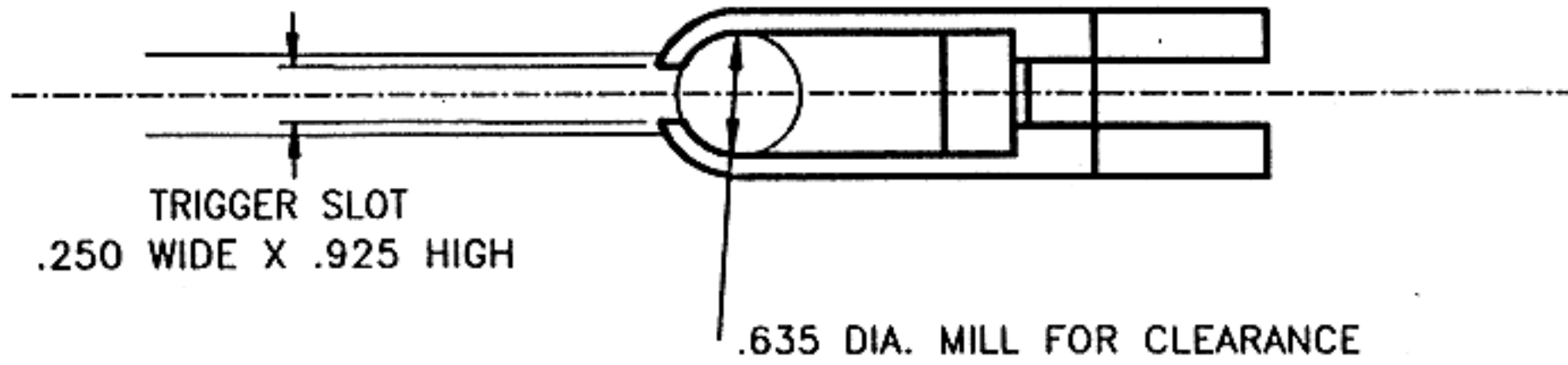
SECTION C-C TRIGGER SECTION
