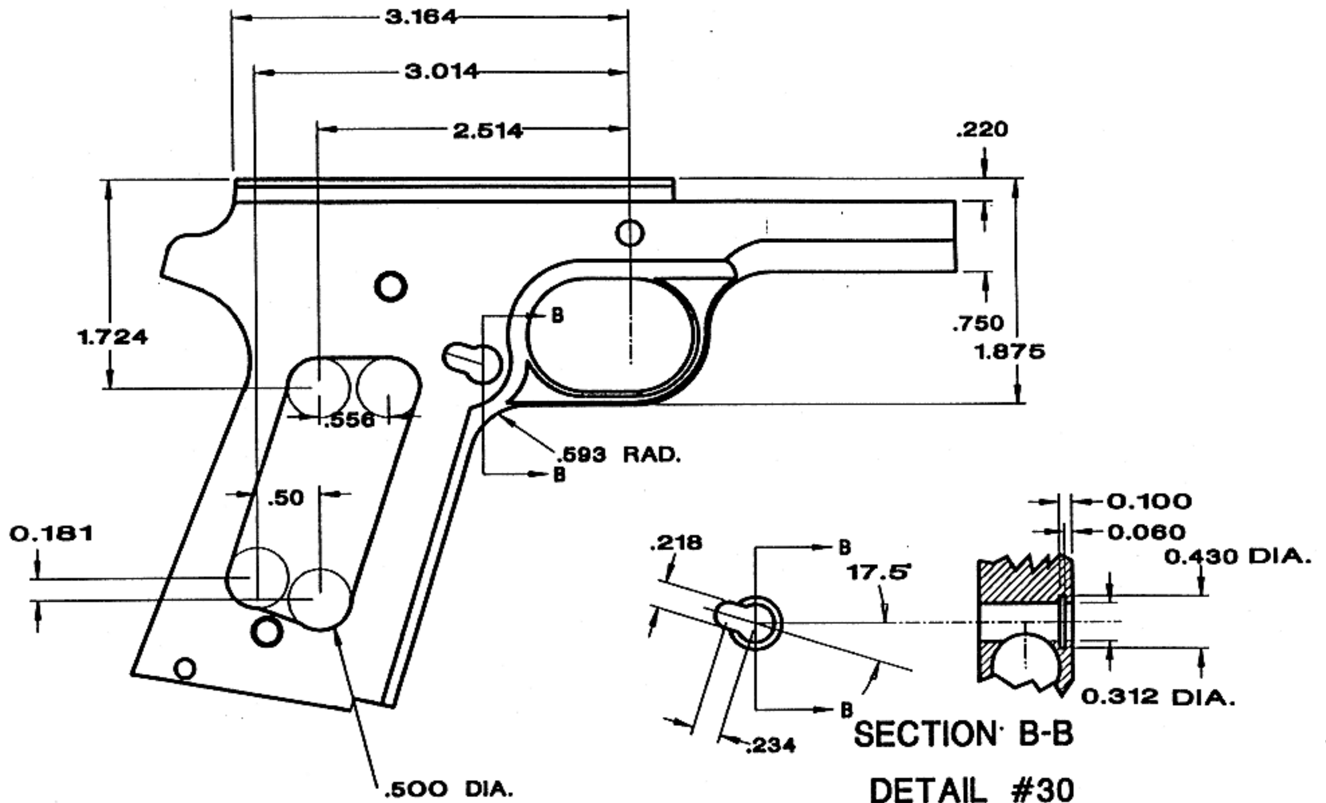
RIGHT SIDE MAG. CATCH DETAIL
