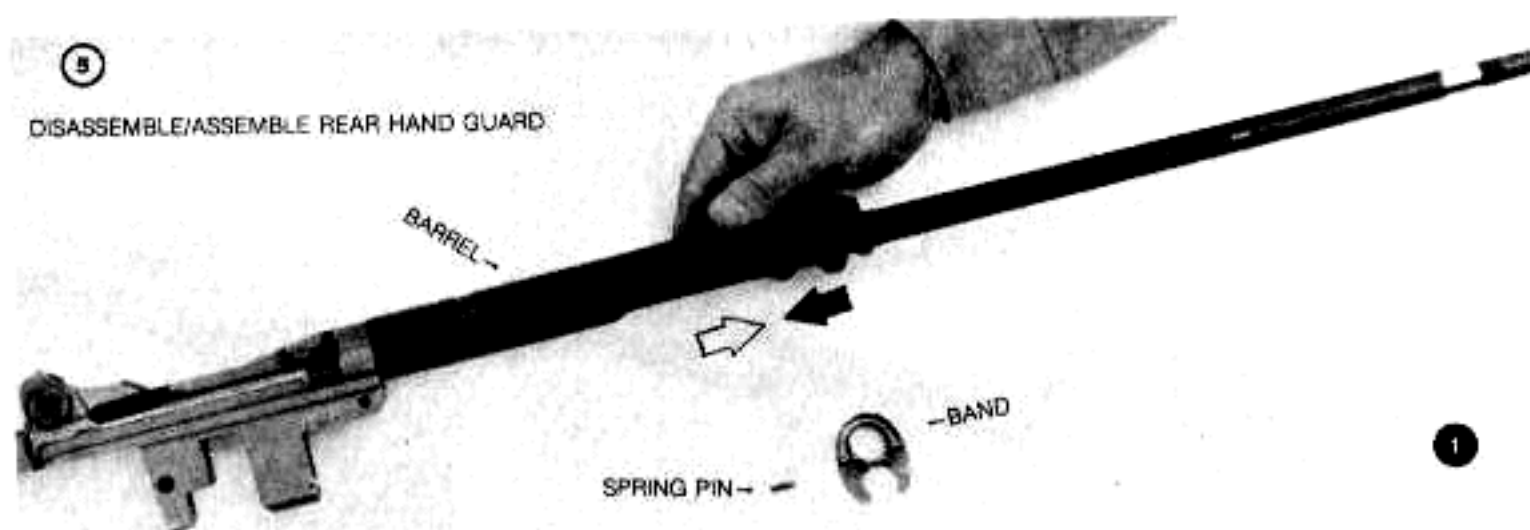
Figure 28. Disassembly / assembly of handguard group (2 of 2).
