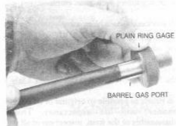
Figure 46. Gaging barrel diameter at gas port.
