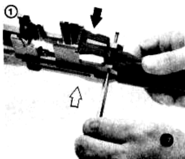
DISASSEMBLE/ASSEMBLE SHOULDER HEADED PIN.
