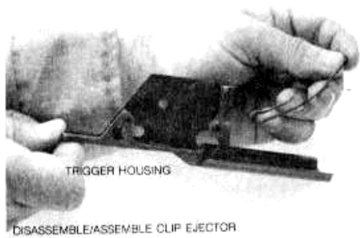
Figure 19. Disassembly / assembly of trigger housing assembly (4 of 4).
