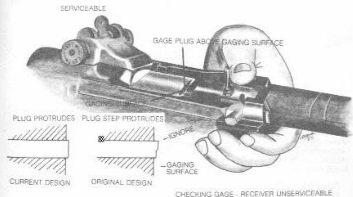
Figure 49. Gaging receiver.
