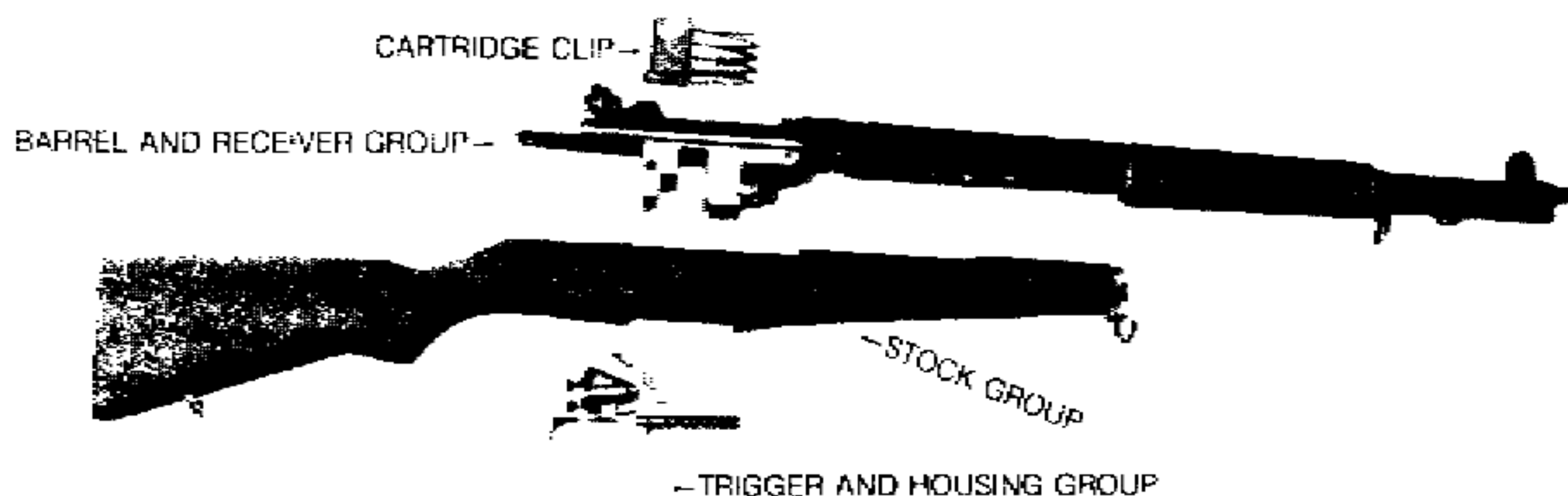
Figure 13. U.S. Rifle, Caliber .30, M 1. Major assembly group.
