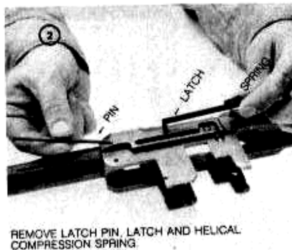
Figure 29. Disassembly / assembly of latch group.
