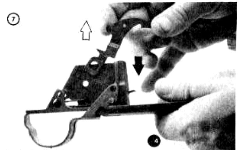
DISASSEMBLE/ASSEMBLE SAFETY
