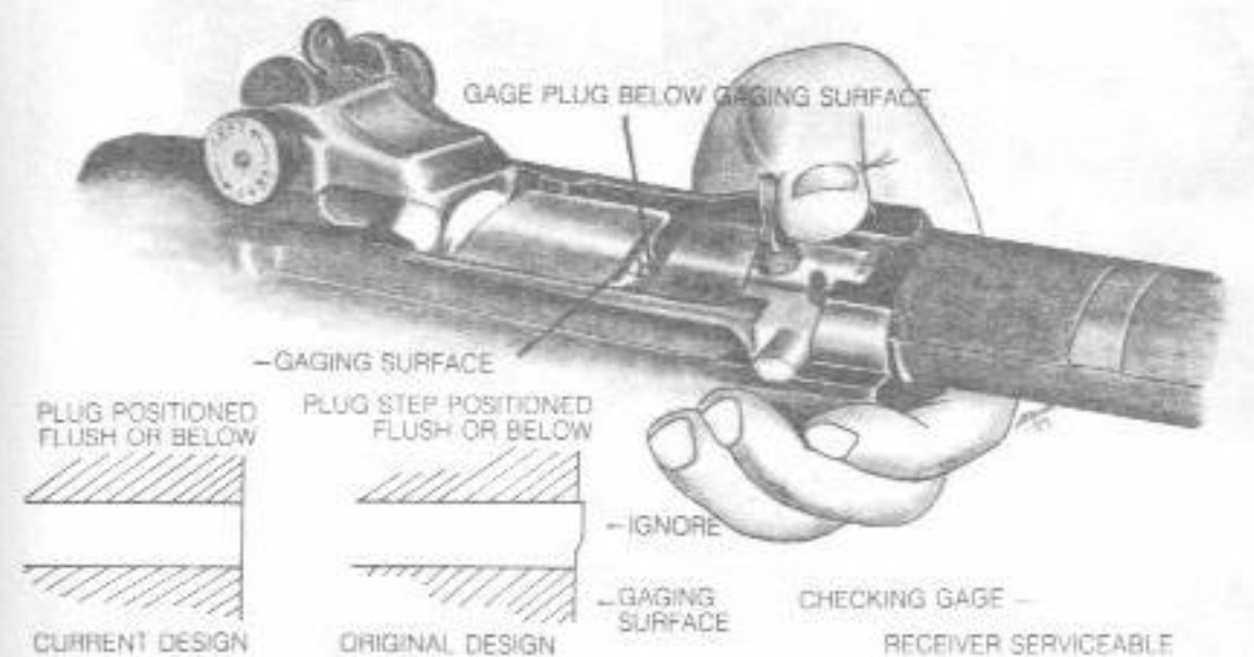
GAGE PROPERLY POSITIONED IN RECEIVER
