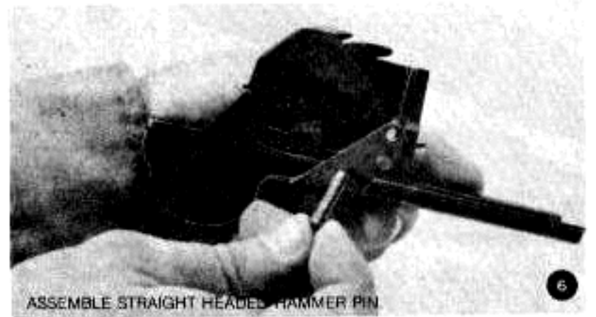
Figure 17. Disassembly / assembly of trigger housing assembly (2 of 4).
