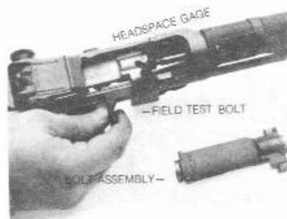
Figure 51. Checking headspace.
