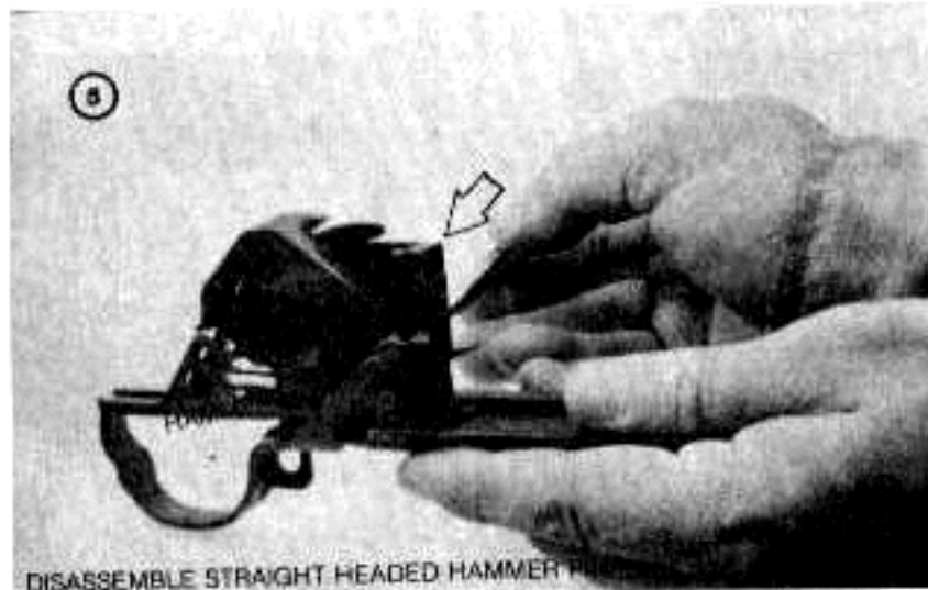
Figure 17. Disassembly / assembly of trigger housing assembly (2 of 4).
