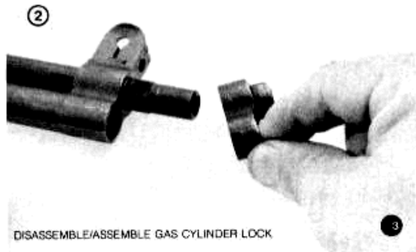
Figure 22. Disassembly / assembly of gas cylinder group (1 of 2).
