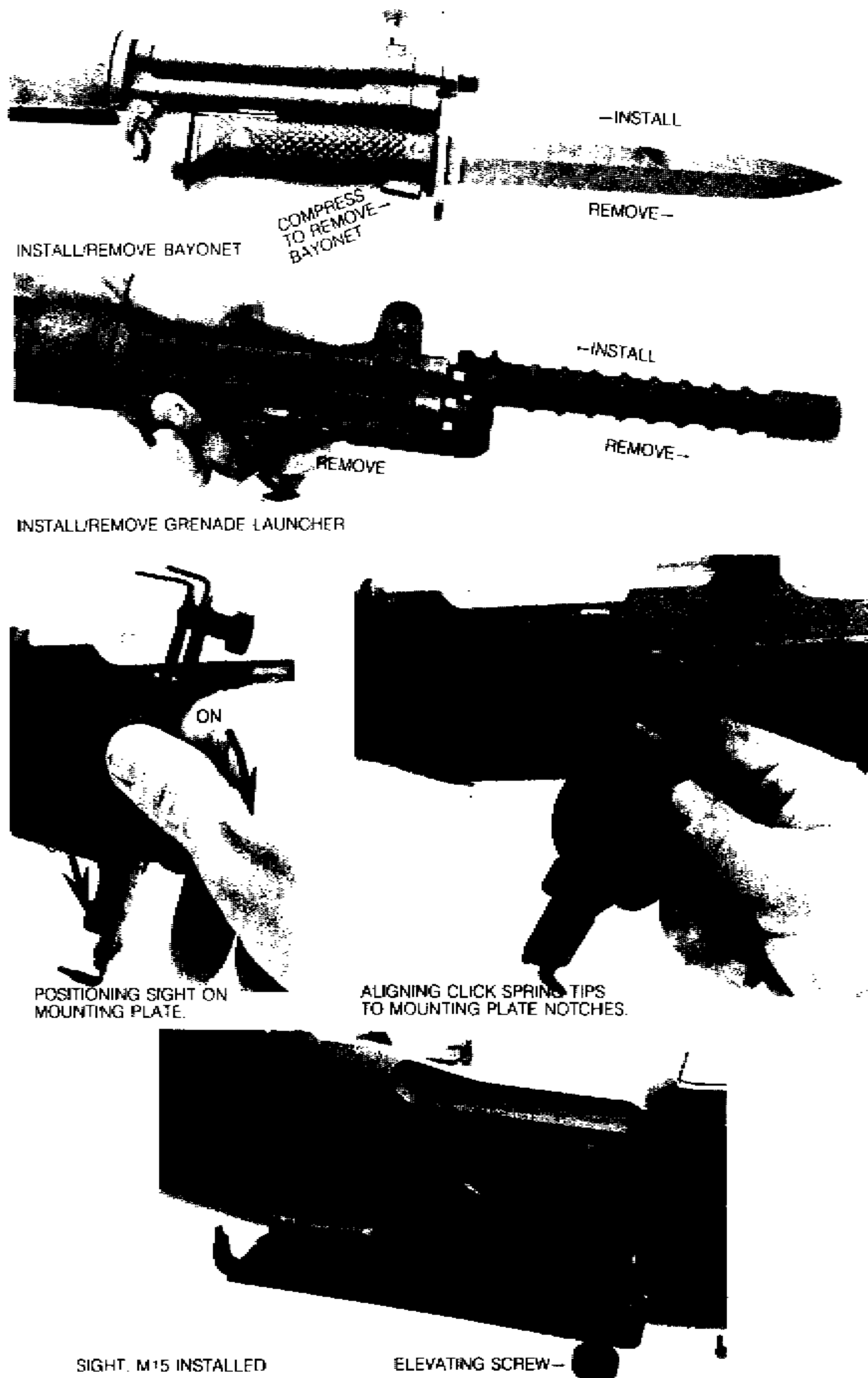
Figure 31. Materiel used in conjunction with major items.
