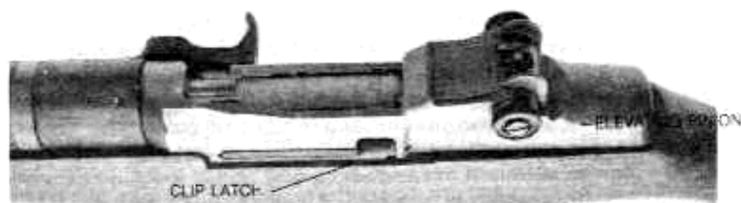
Figure 12. Controls.
