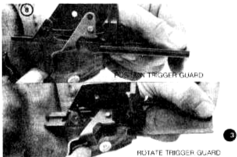
DISASSEMBLE/ASSEMBLE TRIGGER GUARD
