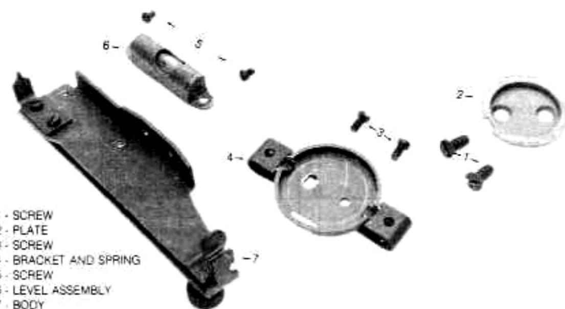
Figure 42. Grenade launcher sight, M 15 - exploded view.
