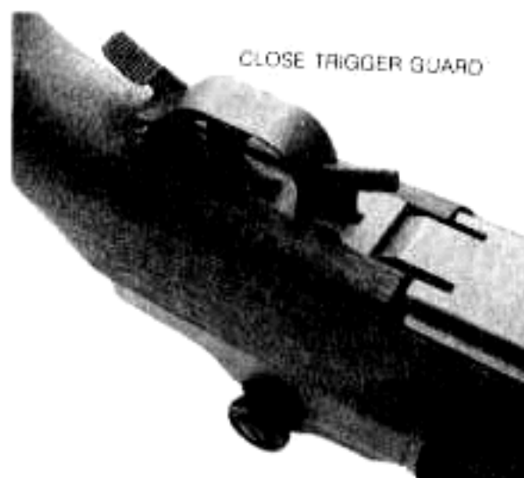
Figure 58. Installation of alternate winter trigger bit. Type T-36
