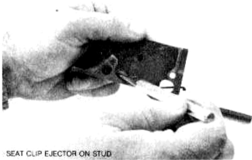
Figure 19. Disassembly / assembly of trigger housing assembly (4 of 4).
