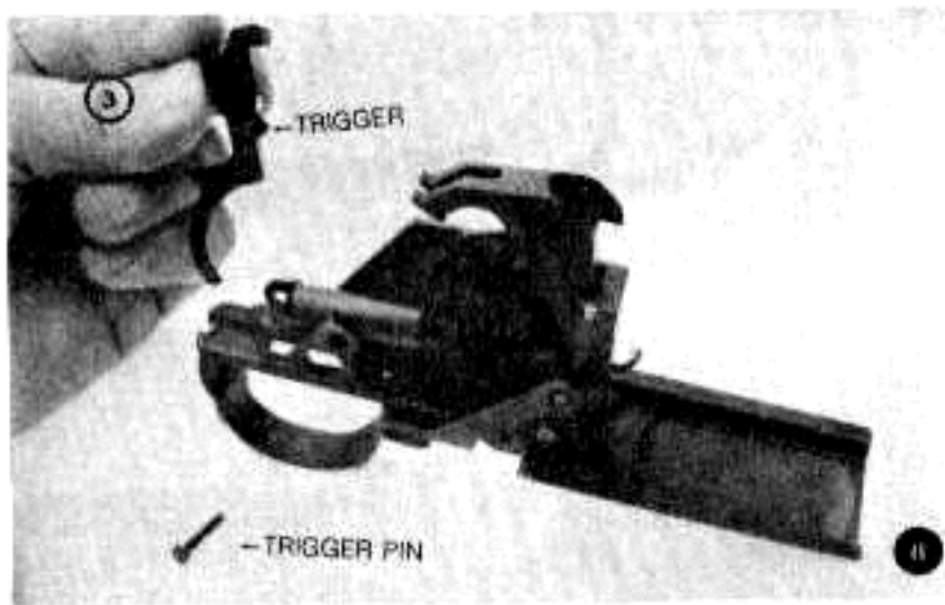
DISASSEMBLE/ASSEMBLE TRIGGER
