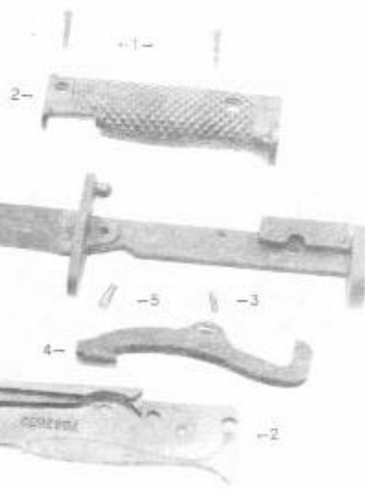
Figure 53. Bayonet knife, M 5A1 - exploded view.
