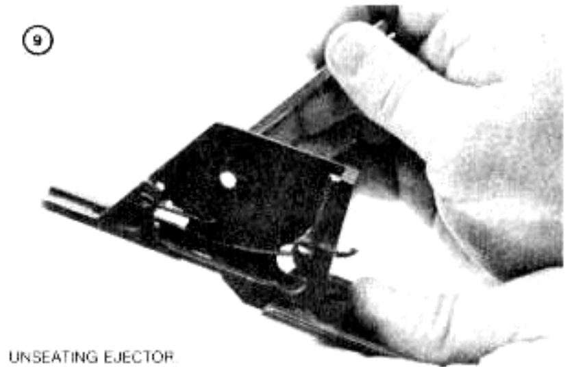
Figure 18. Disassembly / assembly of trigger housing assembly (3 of 4).
