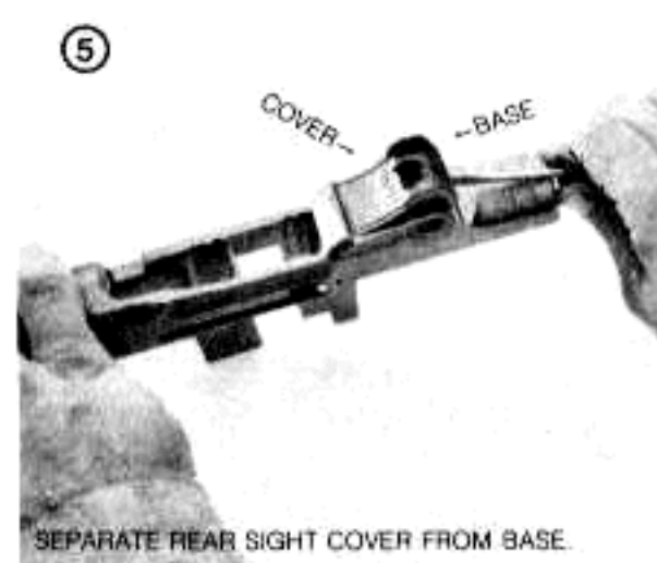
Figure 30. Disassembly / assembly of rear sight group.
