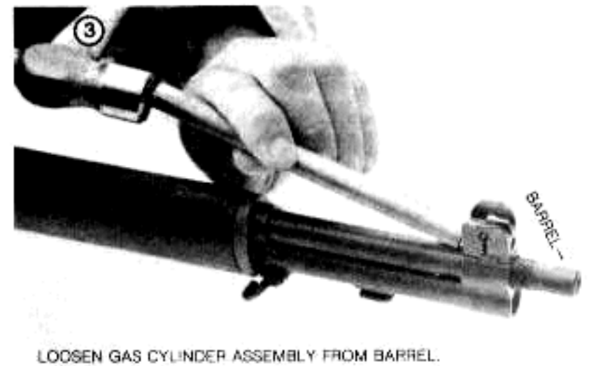
Figure 22. Disassembly / assembly of gas cylinder group (1 of 2).
