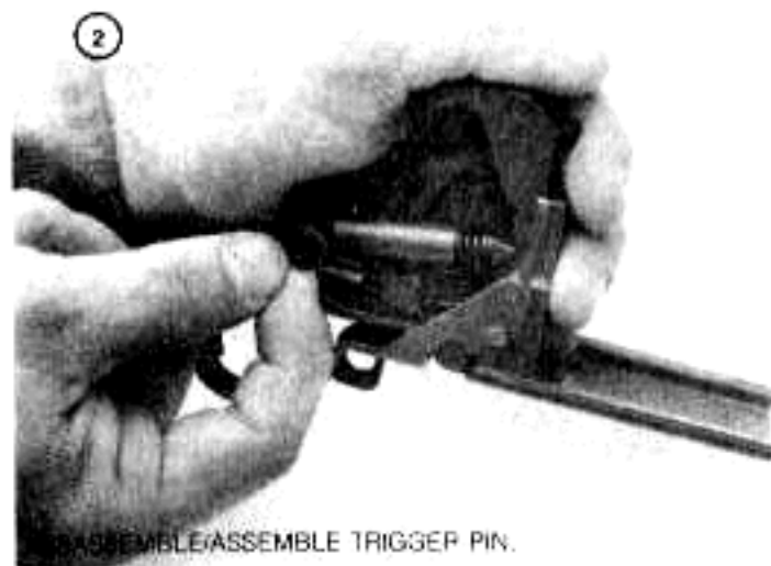
Figure 16. Disassembly / assembly of trigger housing assembly (1 of 4).
