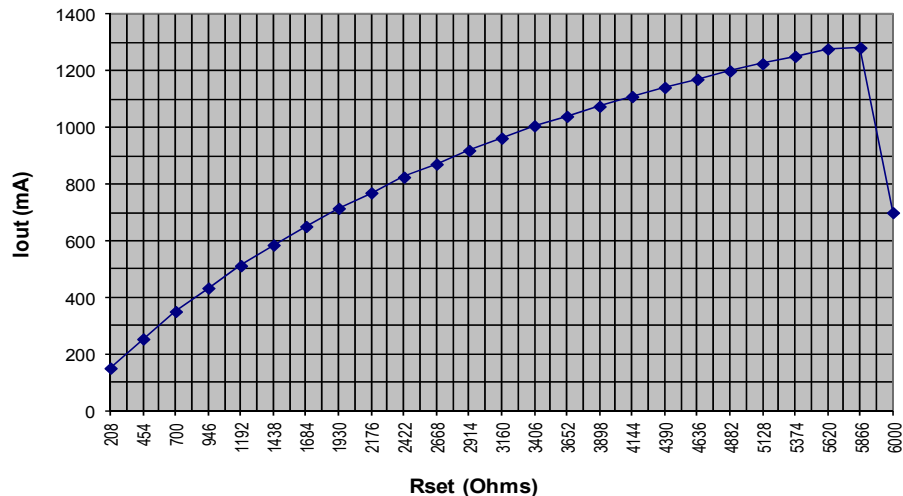
Output Current (mA) vs. Rset (Ohms)
