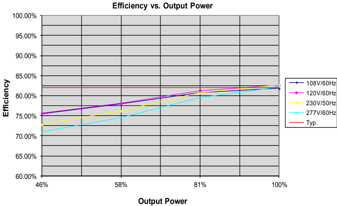
Efficiency Curves (Typical): Vout 26V @ Iout 1500mA
