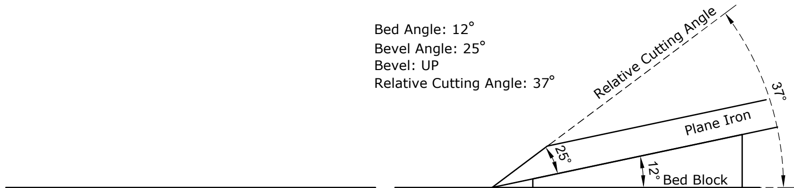
C. Low-Angle Bench or Block Plane
