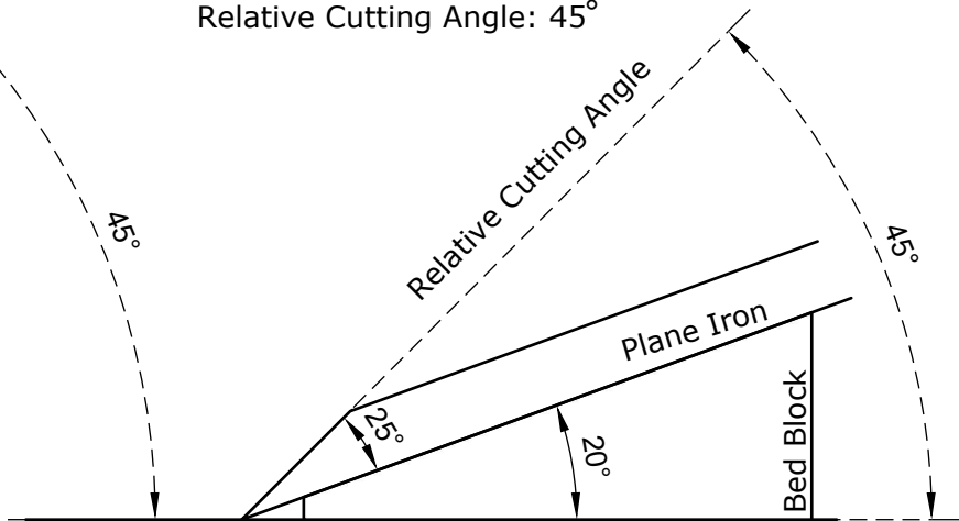
B. Standard Block Plane
