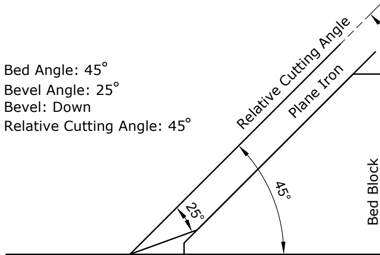
A. Standard Bench Plane
