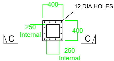
PLAN ON 3-3
