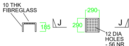
SECTION J-J
