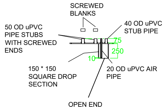
SECTION H-H
