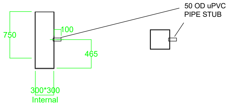
SECTIONAL ELEVATION
