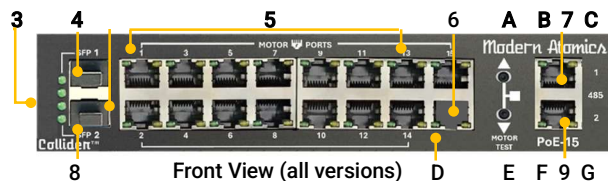
Front View (all versions)
