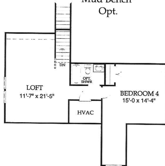
Opt. Loft @ Attic Area with Bedroom and Full Bath Apx. 757 Sq. Ft.
