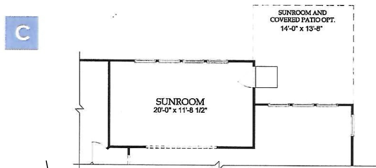
Sunroom Opt. Apx. 242 Sq. Ft.
