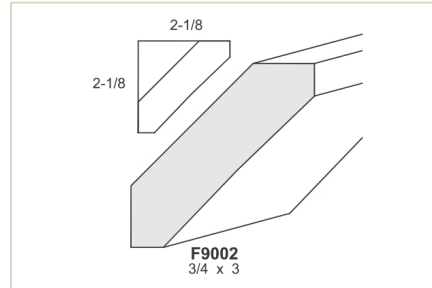
F9002 3/4" x 3" — plain sprung
