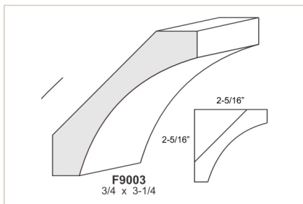
F9003 3/4" x 3-1/4" — cove
