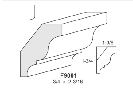
F9001 3/4" x 2-3/16" — petite
