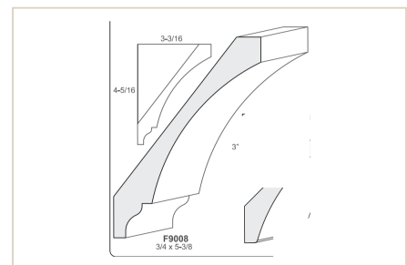
F9008 3/4" x 5-3/8" — estate
