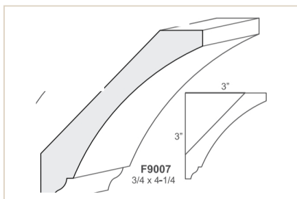
F9007 3/4" x 4-1/4" — cove & bead
